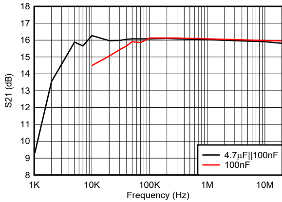
Low frequency cut-off as a function of ac-coupling cap
