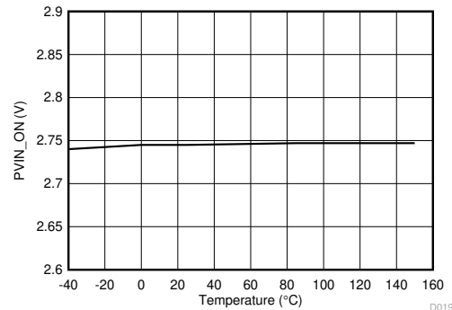
5-14. Turn-On Voltage vs Junction Temperature
