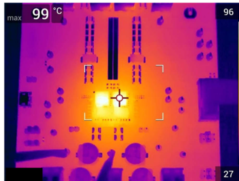
図 7-24. Thermal Image at 25°C Ambient, 12 Vin, 0.8 Vout, 70 A, 550 kHz
