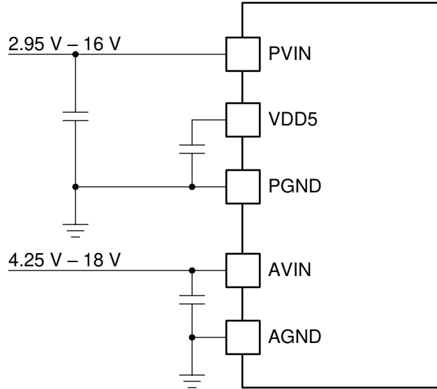
図 6-2. TPSM8D6C24 Separate PVIN and AVIN Connections
