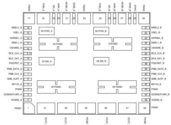
図 4-2. 59-Pin QFM-MOW Package (Bottom View)
