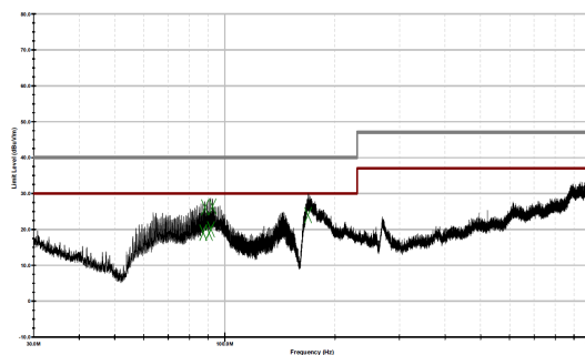
図 7-25. Radiated Emissions 12-V Input, 1.0-V Outputs, 35-A/Output Load
