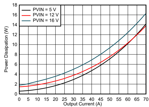
7-13. Power Dissipation
