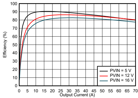
7-10. Efficiency vs Output Current
