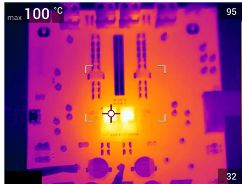
図 7-23. Thermal Image at 25°C Ambient, 12 Vin, 0.8V and 1.2 Vout, 35 A, 550 kHz
