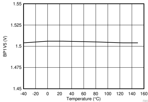
5-13. BP1V5 Voltage vs Junction Temperature
