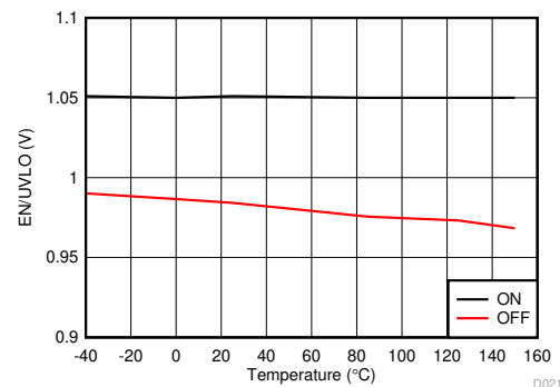
5-16. EN/UVLO Thresholds vs Junction Temperature
