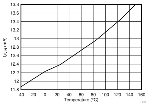
图 5-11. Nonswitching Input Current ( I_{AVIN} ) vs Junction Temperature
