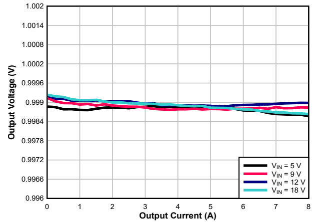
7-5. Load Regulation
