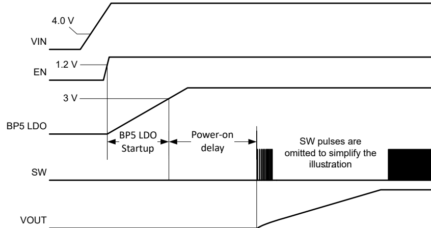
図 6-1. Start-Up Sequence
