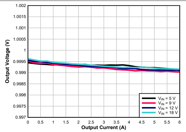
7-5. Load Regulation
