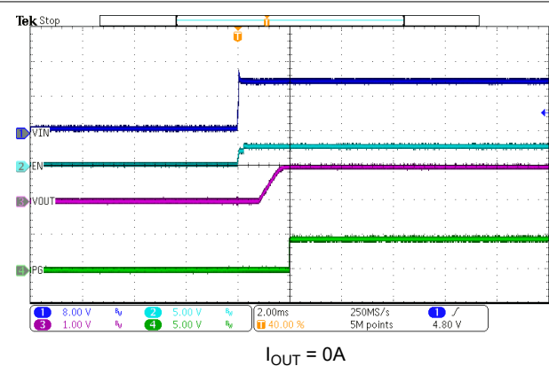
7-13. VIN Start-Up
