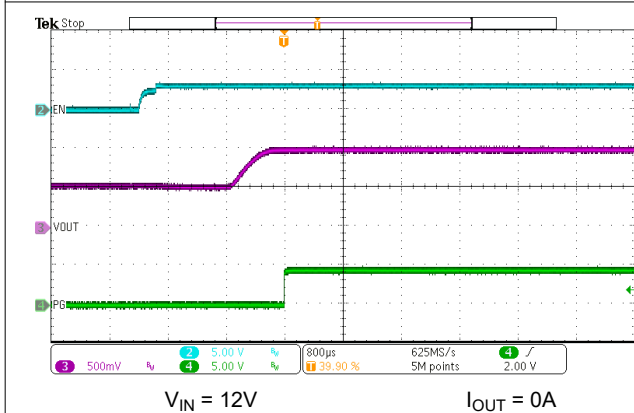
7-12. EN Start-Up – 0.5V Prebias
