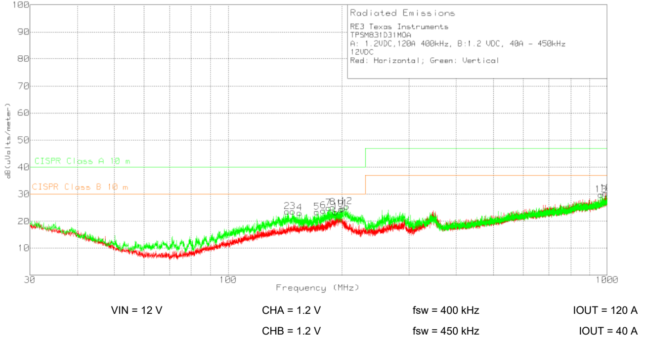
8-16. Radiated EMI
