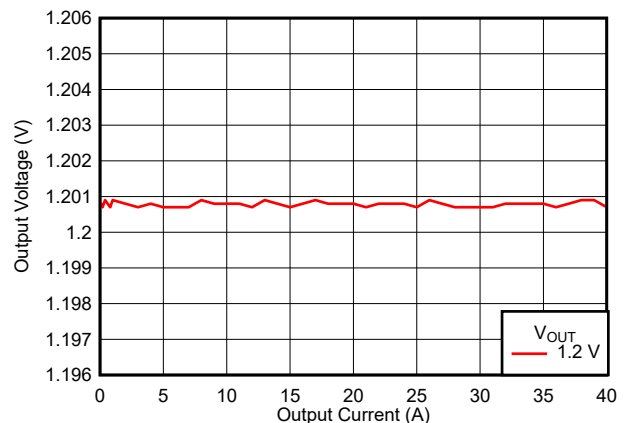
8-7. VOUTB Load Regulation
