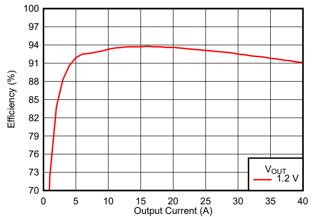
8-3. VOUTB Efficiency
