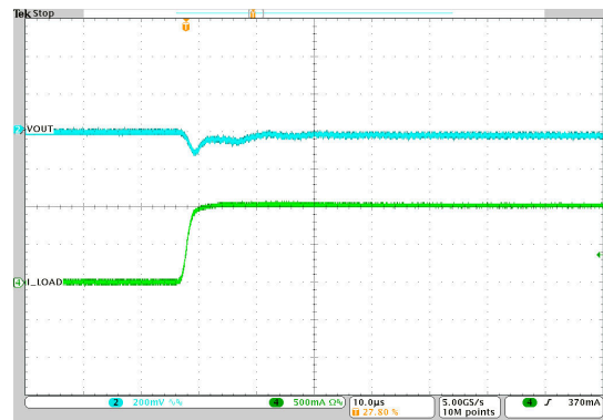
8-38. PSM-to-PWM Transition
