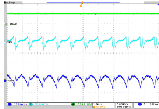
V_{IN} = 12\text{ V} 1-MHz Auto I_O = 2\text{ A} PFM/PWM V_{OUT} = 1.2\text{ V} T_A = 25^\circ\text{C}
