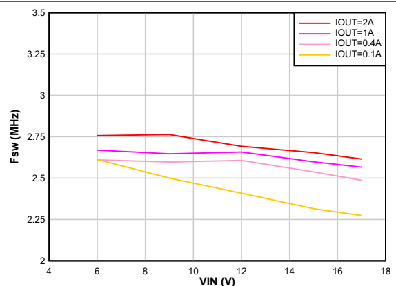
8-20. Switching Frequency vs Input Voltage V_{OUT} = 1.2\text{ V}
