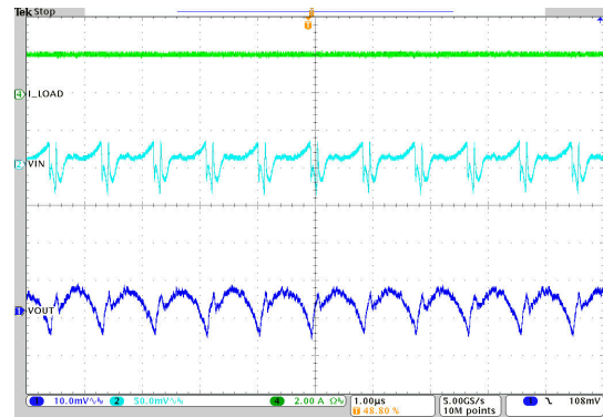
V_{IN} = 12\text{ V} 2.5-MHz Auto I_O = 2\text{ A} PFM/PWM V_{OUT} = 1.2\text{ V} T_A = 25^\circ\text{C}
