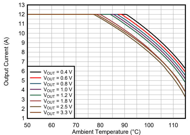
9-41. Safe Operating Area TPSM8287A10BAH V_{IN} = 5.0\text{ V}
