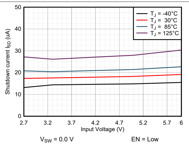
6-2. Shutdown Current
