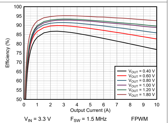
9-5. Efficiency TPSM8287A10BAH
