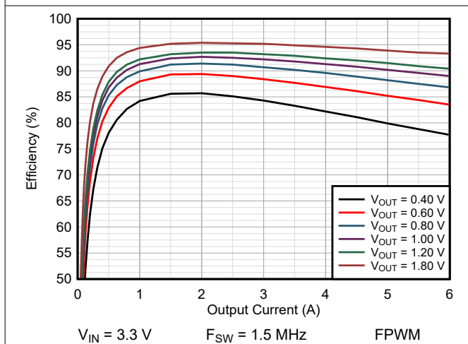
9-4. Efficiency TPSM8287A06BAS
