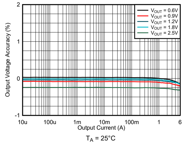
8-23. Load Regulation V_{IN} = 3.3\text{ V} and FPWM
