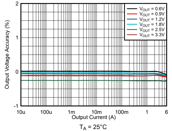
8-21. Load Regulation V_{IN} = 5.0\text{ V} and FPWM
