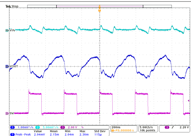
8-31. FPWM Operation I_{OUT} = 0.1\text{ A}
