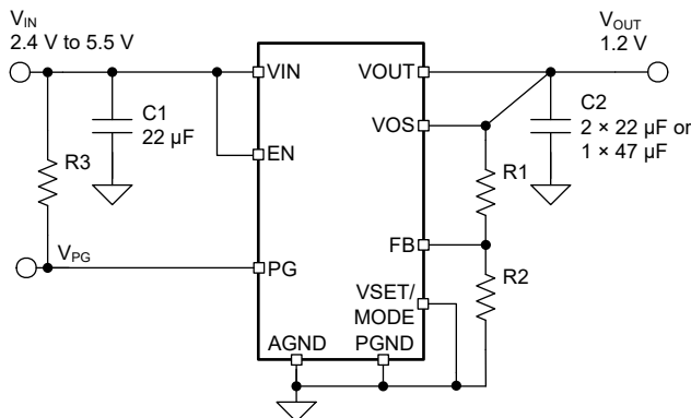
図 8-1. Typical Application
