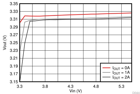
9-73. Line Regulation
