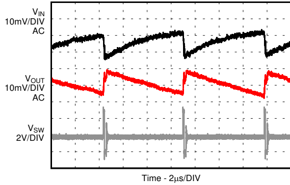
I_{OUT} = 25 \text{ mA} TPSM82822
