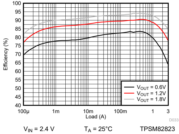
9-116. Efficiency
