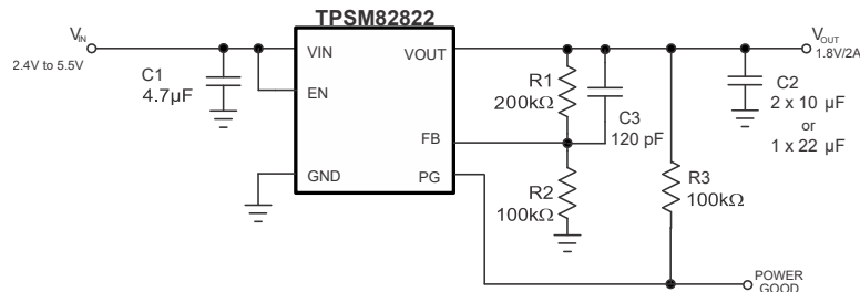
☒ 9-1. Adjustable Output Application Set at 1.8-V Output Voltage
