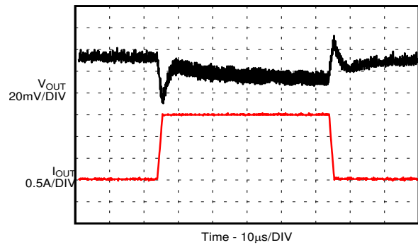
I_{OUT} = 0.5 \text{ A to } 2 \text{ A} Slew Rate = 2 \text{ A}/\mu\text{s} TPSM82822
