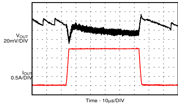
I_{OUT} = 0 \text{ A to } 2 \text{ A} Slew Rate = 2 \text{ A}/\mu\text{s} TPSM82822
