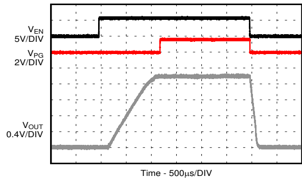
I_{OUT} = \text{no load} TPSM82822
