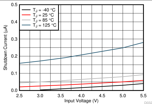
Figure 7-5. Shutdown Current
