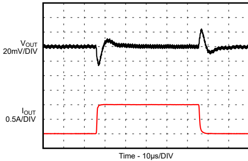
I_{OUT} = 0\text{ A to }1\text{ A} Slope Rate = 2\text{ A}/\mu\text{s} TPSM82821A
