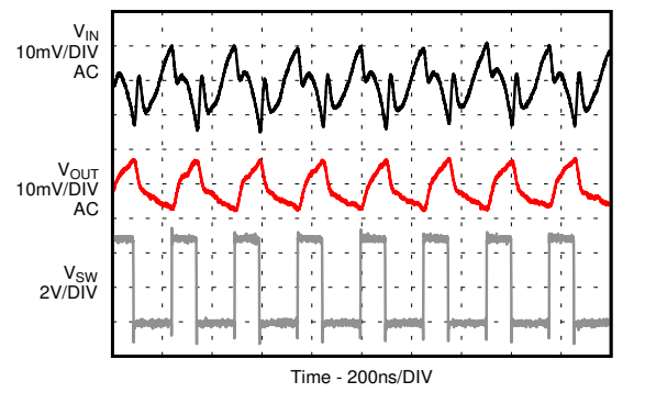
9-76. Input and Output Ripple in PWM Mode
