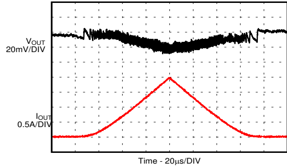
I_{OUT} = 25 \text{ mA to } 2 \text{ A} TPSM82822
