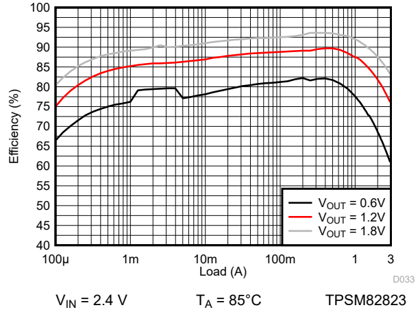
9-117. Efficiency
