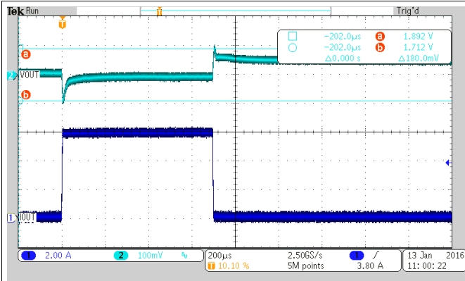
34. Load Transient Response (PWM-PWM), Load Step 0 to 6 A
