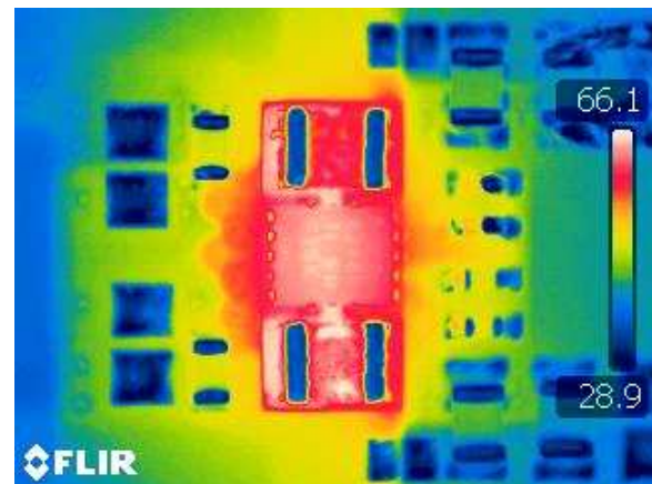
37. Device Temperature (TPSM82480 EVM)
