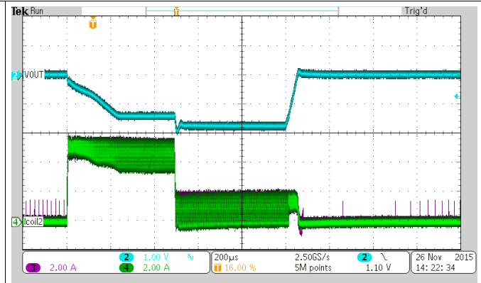
35. Current Limit Fold-Back at Overload
