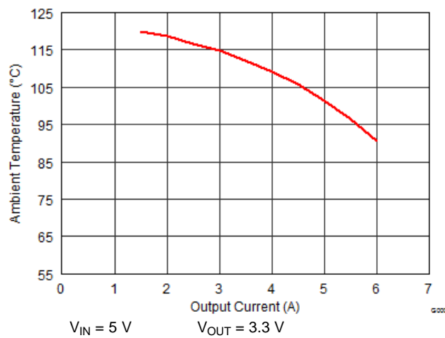
36. Maximum Ambient Temperature for T_J=125^\circ\text{C} (TPSM82480 EVM)
