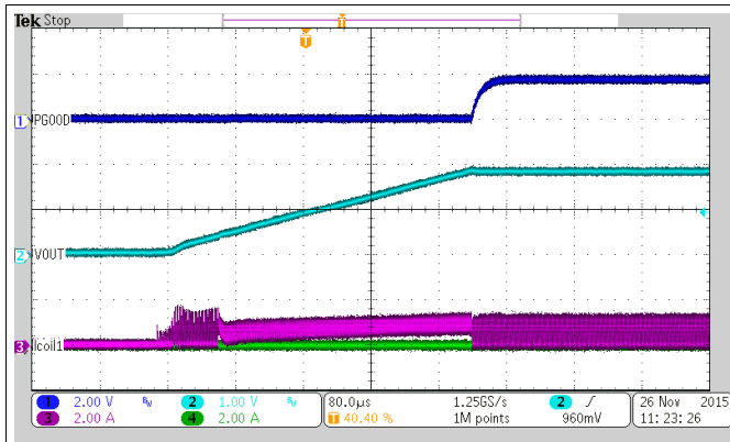
22. Startup into 3.3 \Omega resistor
