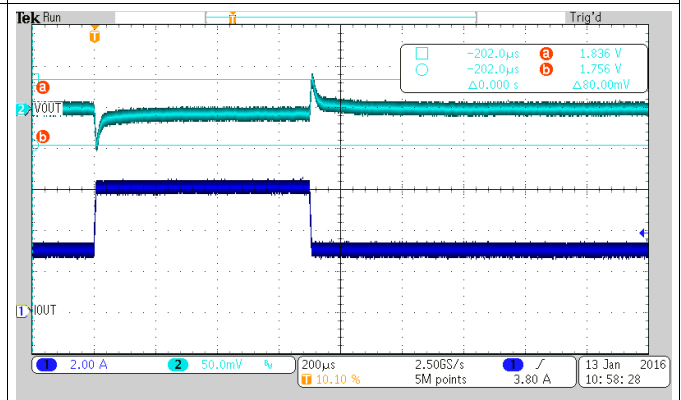
31. Load Transient Response (PSM-PWM), Load Step 0 to 3 A
