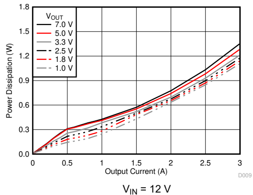
6-9. Power Dissipation versus Output Current
