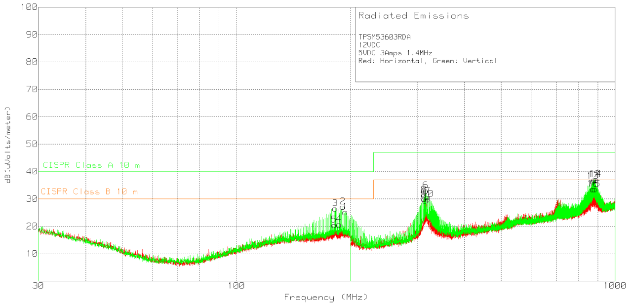
10-6. Radiated Emissions 12-V Input, 5-V Output, 3-A Load
