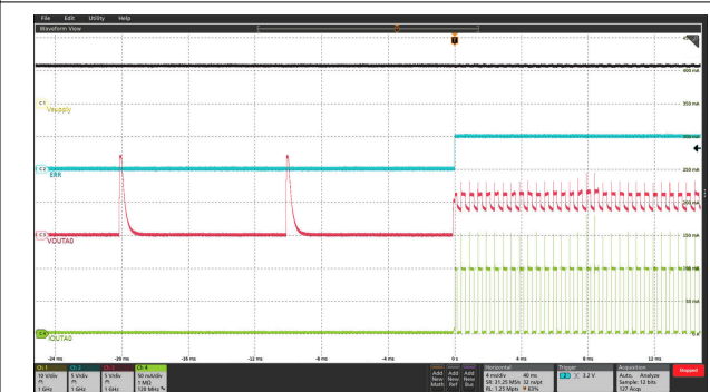
5-27. Single-LED Short-Circuit Detection in Normal Mode
