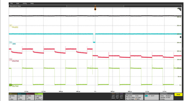
5-25. LED Open-Circuit Detection in Normal Mode
