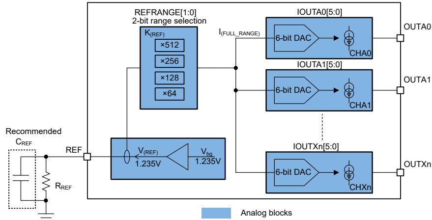
6-1. Output Current Setting
