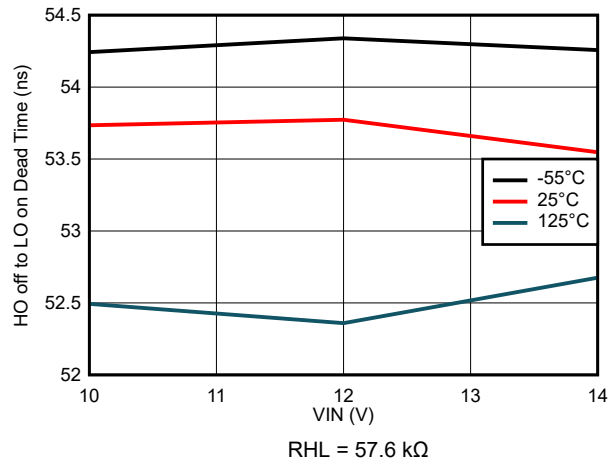
7-38. HO off to LO on Dead Time vs VIN Voltage
