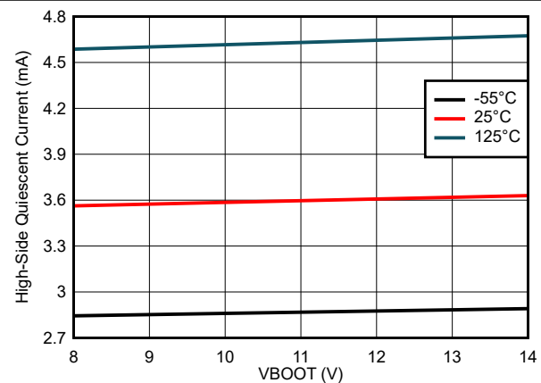
7-41. High-Side Quiescent Current vs BOOT Voltage
