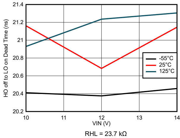
7-37. HO off to LO on Dead Time vs VIN Voltage
