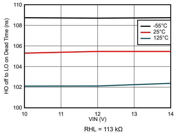
7-39. HO off to LO on Dead Time vs VIN Voltage
