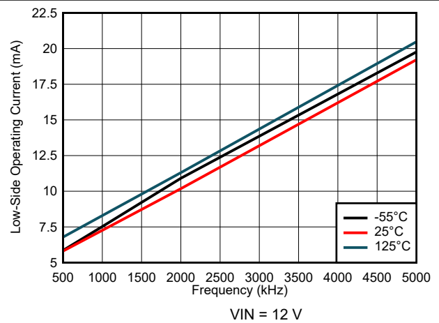
7-42. Low-Side Operating Current vs Frequency (IIM)
