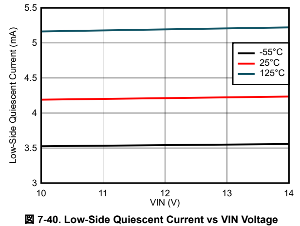
7-40. Low-Side Quiescent Current vs VIN Voltage
