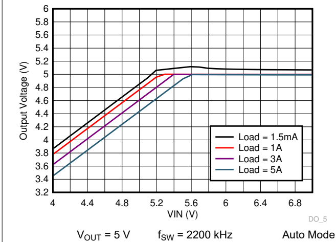
8-11. TPS7H4010-SEP Dropout Curve
