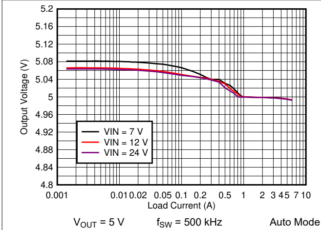
8-9. TPS7H4010-SEP Load and Line Regulation
