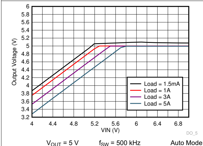
8-13. TPS7H4010-SEP Dropout Curve
