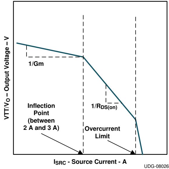
8-9. TPS7H3301-SP Impedance Characteristics
