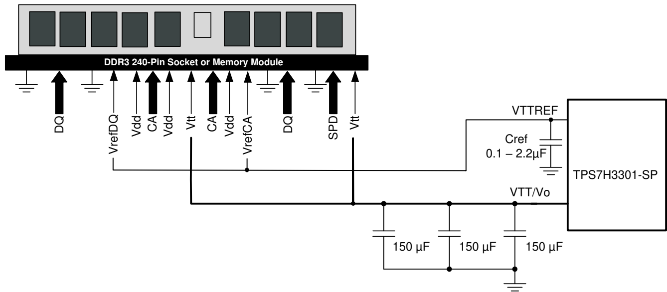
8-5. Typical Application Diagram for DDR3 VTT DIMM/Module Using TPS7H3301-SP
