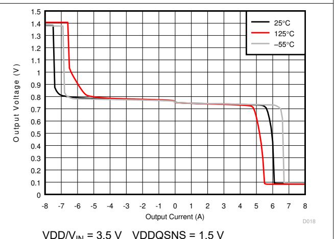
Figure 6-12. Output Voltage vs Output Current, DDR3
