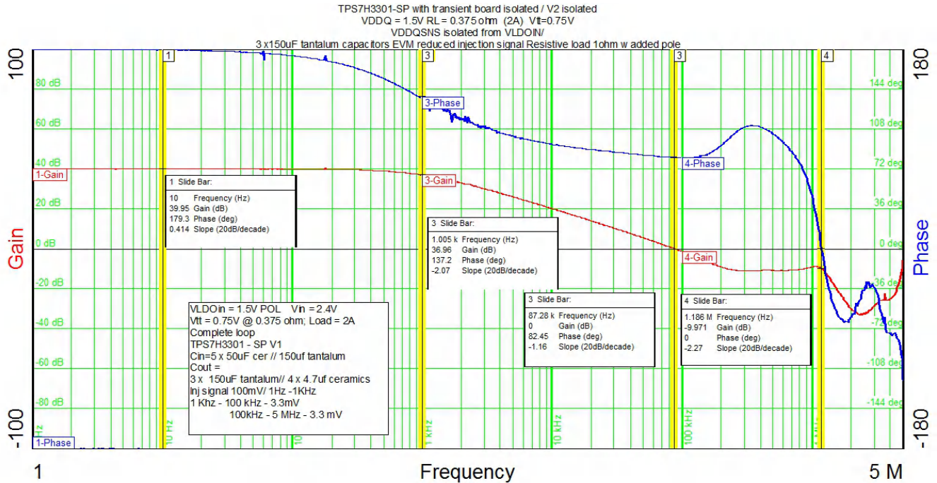
8-7. Bode Plot for a Typical DDR3 Configuration
