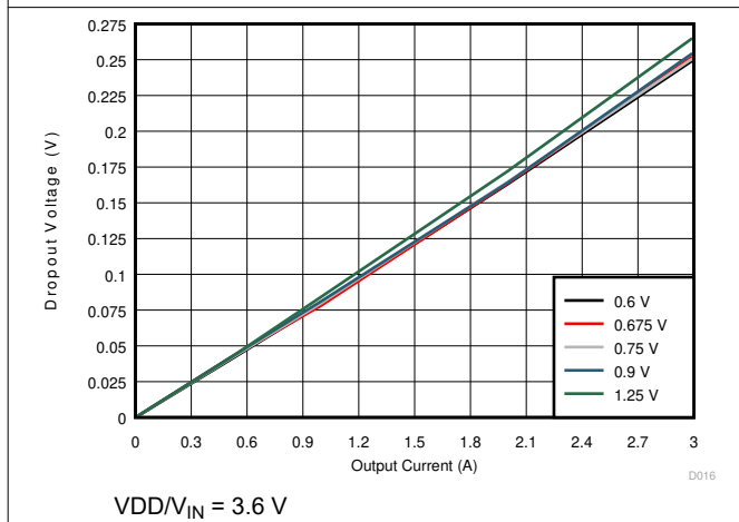
Figure 6-11. Dropout Voltage vs Output Current
