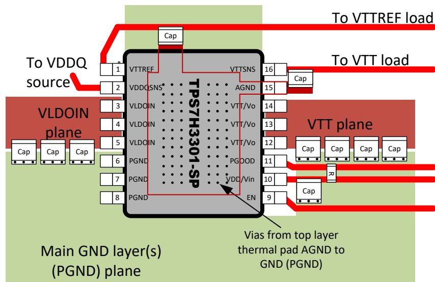
図 9-1. Layout Recommendation
