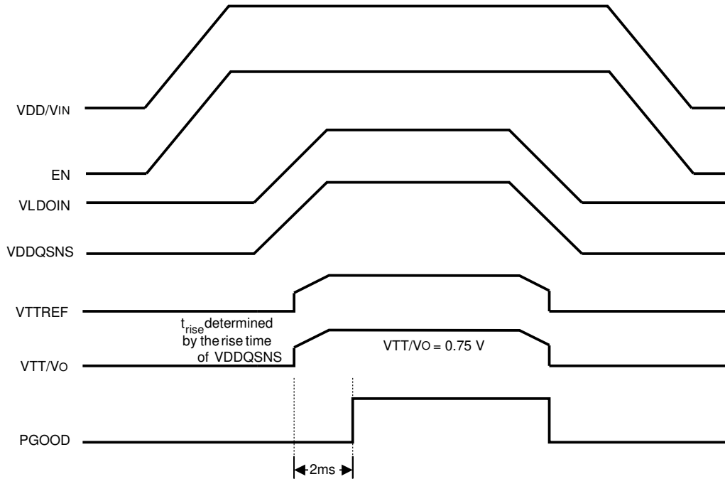
8-4. Typical Timing Diagram of Tracking Startup and Shutdown
