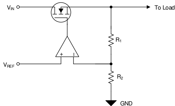
7-3. Simplified Regulation Circuit
