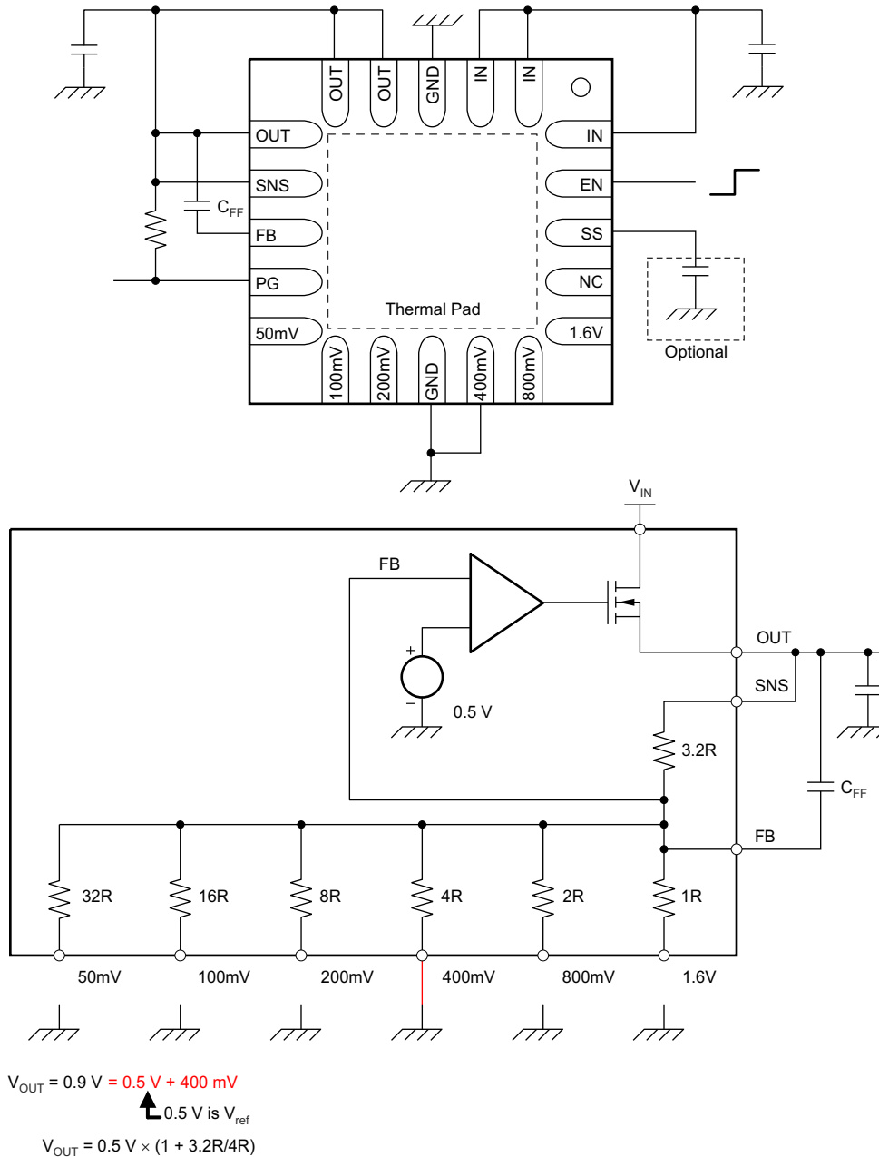
6-1. 0.9-V Configuration
