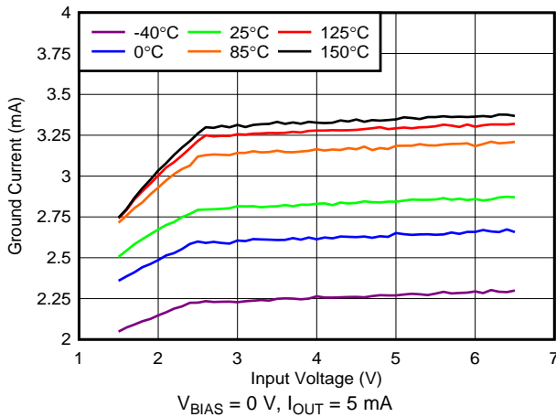
27. Quiescent Current vs Input Voltage
