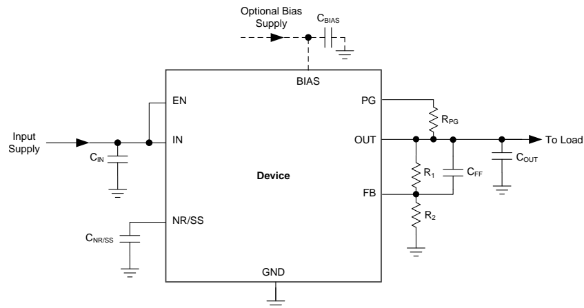
47. Typical Application for a 0.9-V Rail
