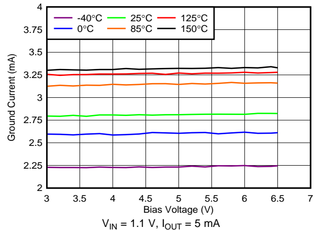
28. Quiescent Current vs Bias Voltage
