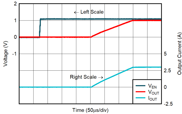
6-13. Start-Up Waveform for C_{SS} = 1\text{ nF}
