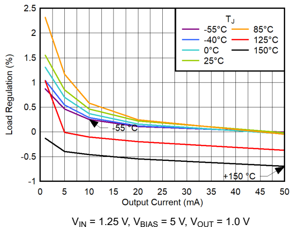
6-21. Load Regulation vs 0-mA to 50-mA Output Current
