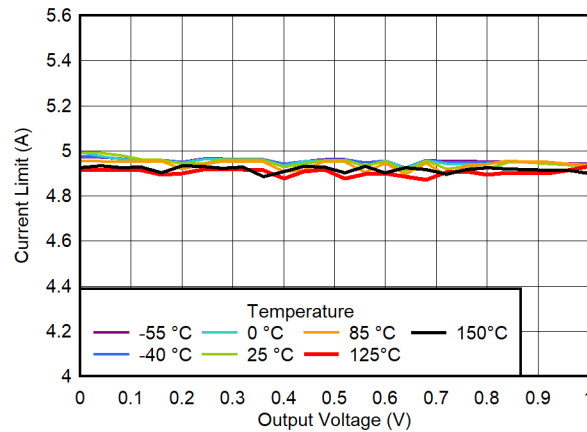
6-31. Current Limit vs Output Voltage
