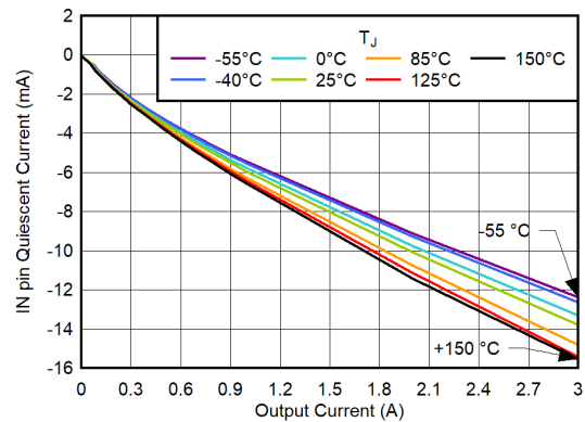
6-26. IN Pin Quiescent Current vs Output Current
