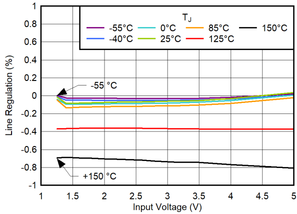
6-23. Line Regulation vs Input Voltage
