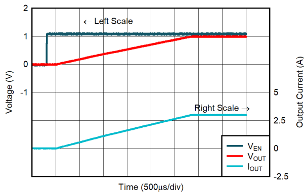
6-13. Start-Up Waveform for C_{SS} = 1\text{ nF}
