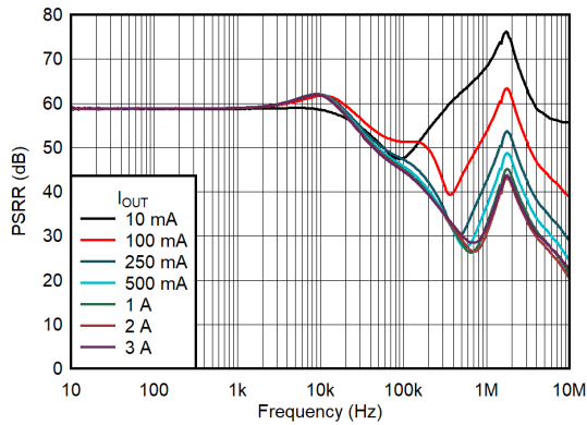
6-7. BIAS PSRR vs Frequency and I_{OUT}
