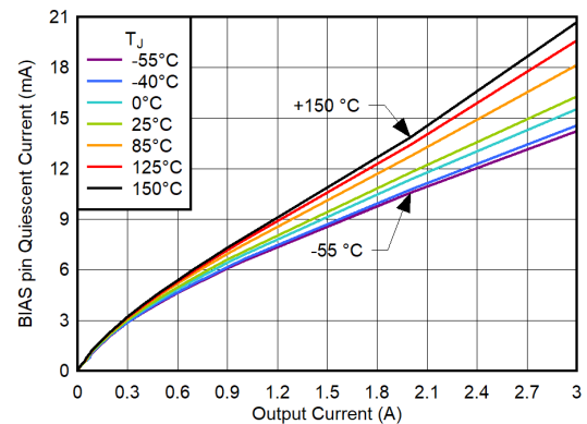
6-28. BIAS Pin Quiescent Current vs Output Current
