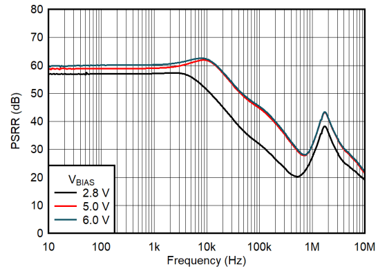
6-8. BIAS PSRR vs Frequency and V_{BIAS}
