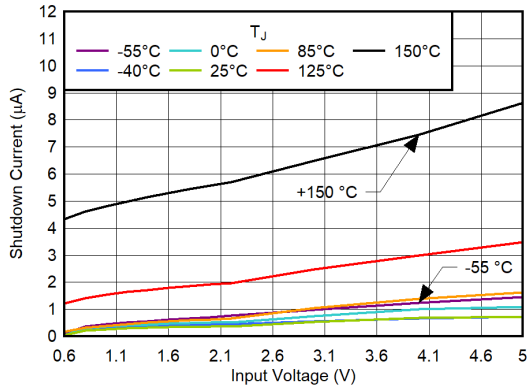
6-29. Shutdown Current (GND Pin) vs Input Voltage
