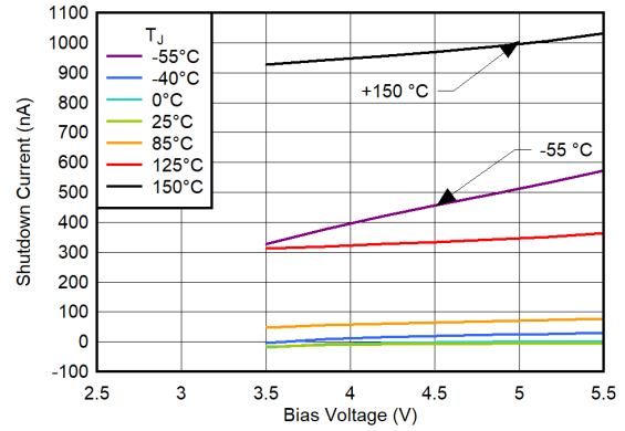
6-30. Shutdown Current (GND Pin) vs Bias Voltage
