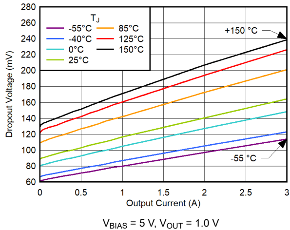
6-19. IN-to-OUT Dropout Voltage vs Output Current
