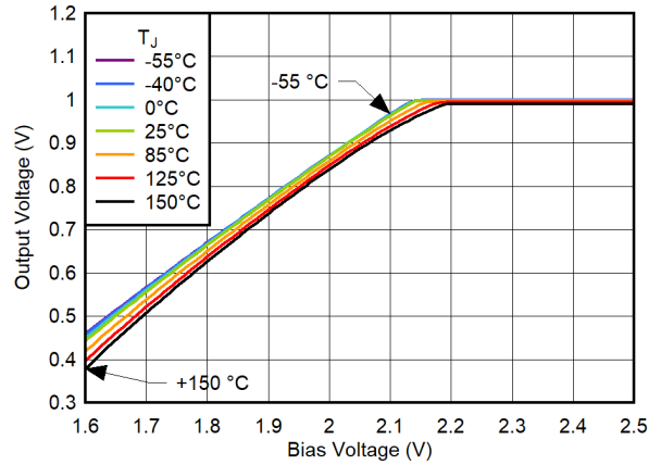
6-24. Output Voltage vs Bias Voltage
