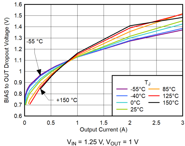
6-20. BIAS-to-OUT Dropout Voltage vs Output Current
