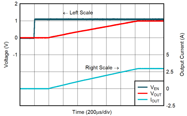
6-14. Start-Up Waveform vs Time for C_{SS} = 10\text{ nF}
