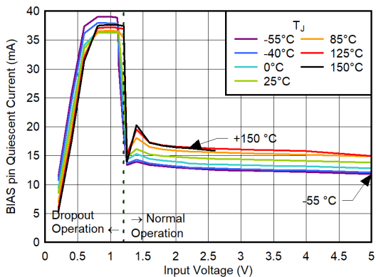
6-27. BIAS Pin Quiescent Current vs Input Voltage
