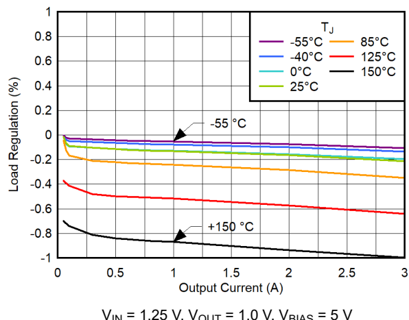
6-22. Load Regulation vs ≥50-mA Output Current
