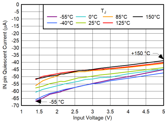
6-25. IN Pin Quiescent Current vs Input Voltage
