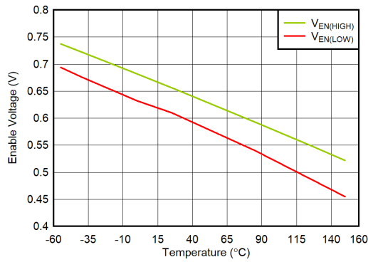
5-15. Enable Logic Threshold vs Temperature
