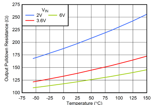
5-18. Output Pulldown Resistance vs Temperature and V_{IN}
