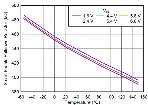
5-17. Smart Enable Pulldown Resistor vs Temperature and V_{IN}
