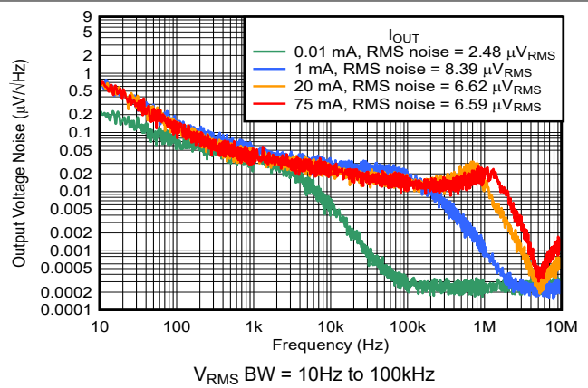
5-30. Noise vs Frequency and I_{OUT}
