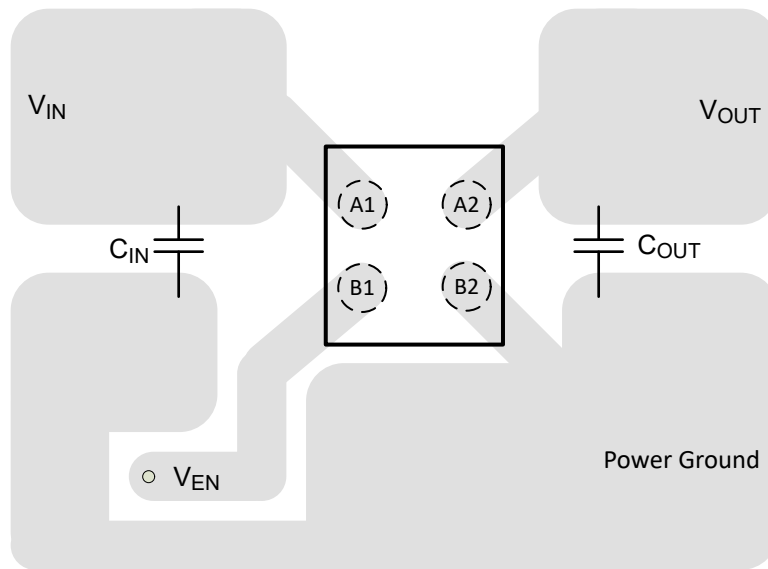
図 7-6. YCK Package (DSBGA) Typical Layout
