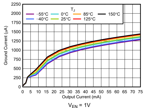
图 5-12. I_{GND} vs I_{OUT}
