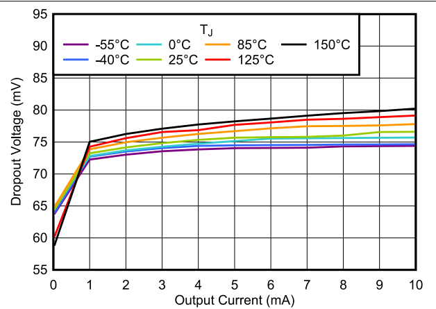
5-28. Dropout Voltage vs I_{OUT}
