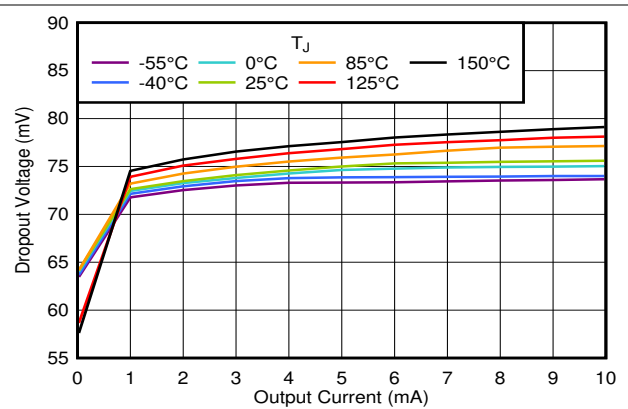
5-26. Dropout Voltage vs I_{OUT}
