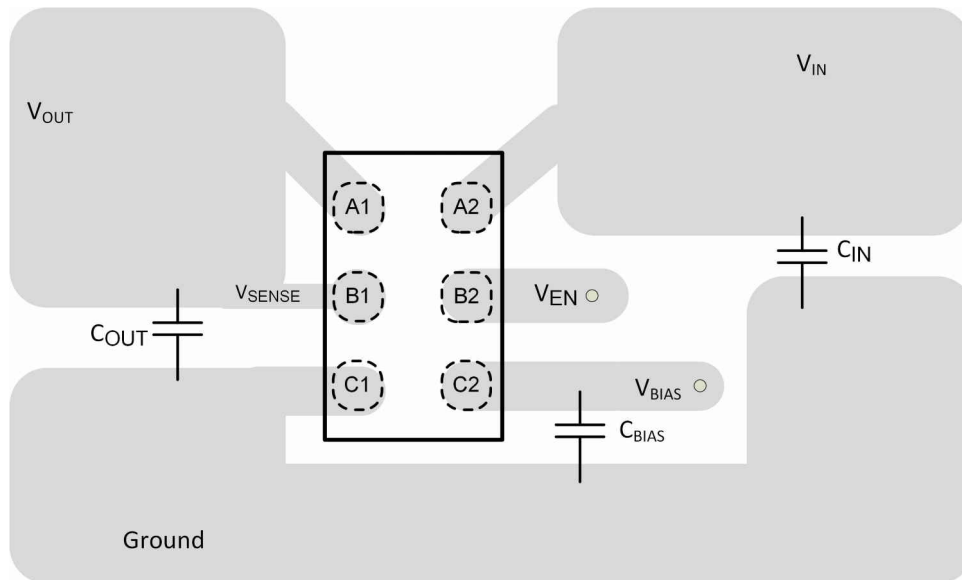
☒ 10-1. Recommended Layout
