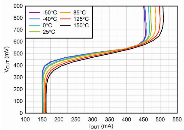
6-10. Foldback Current Limit vs I_{\text{OUT}}
