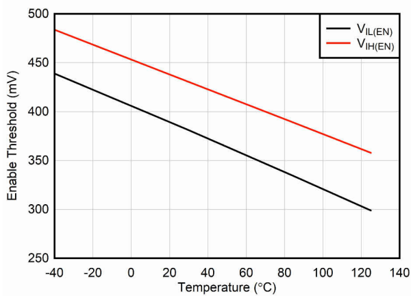
6-11. Enable Threshold vs Temperature
