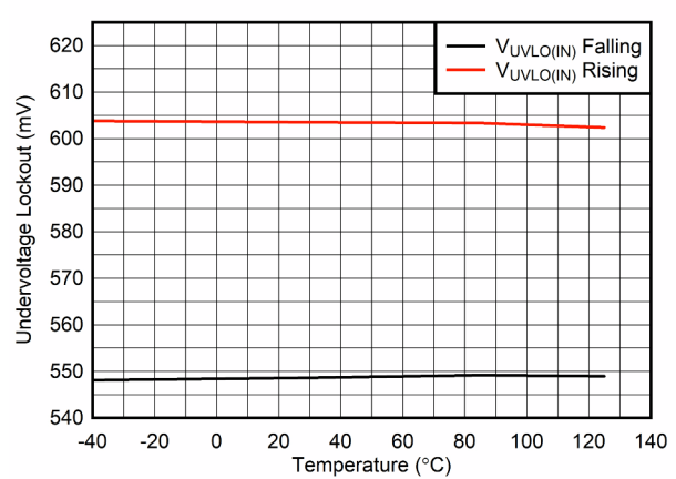
6-12. V_{\text{IN}} UVLO vs Temperature
