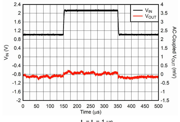
6-18. Line Transient From 1 V to 2.2 V
