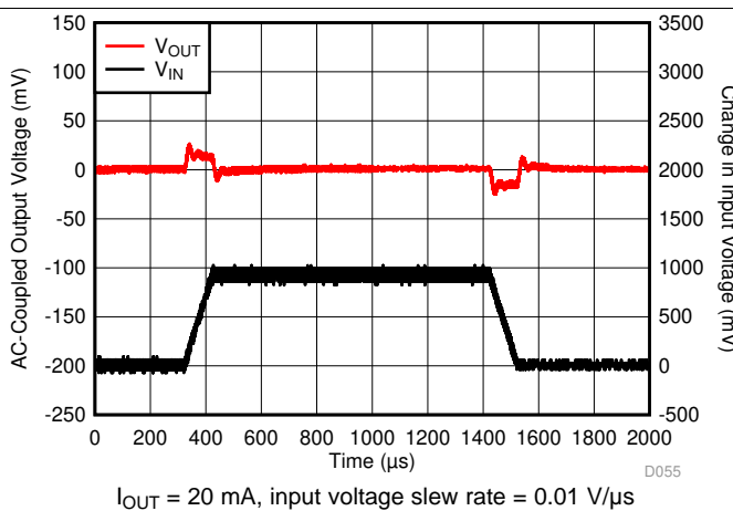
Figure 20. V_{IN} Transient
