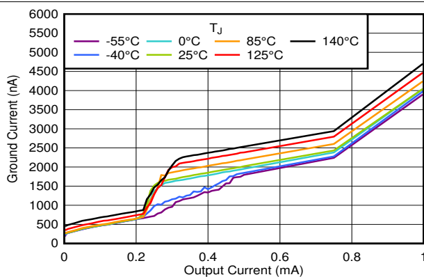
6-5. I_Q vs I_{OUT} and Temperature Up to 1 mA
