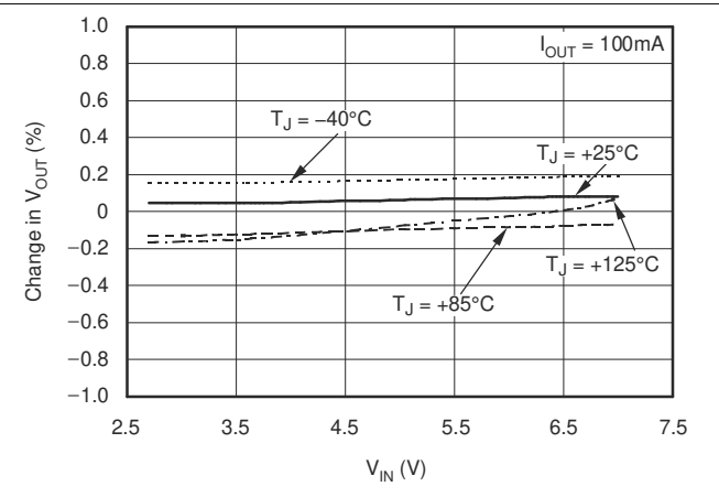
6-2. Line Regulation
