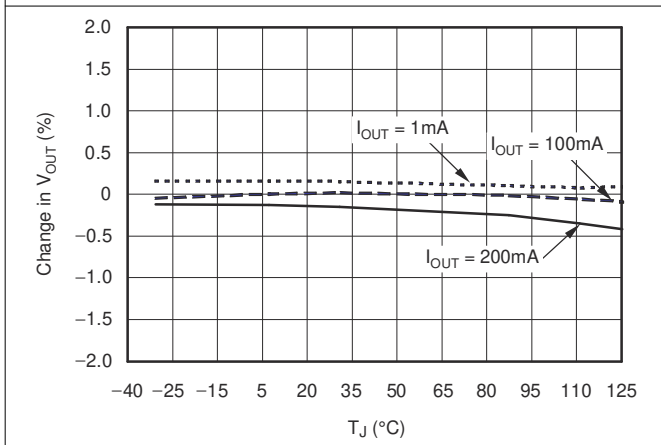
6-1. Load Regulation
