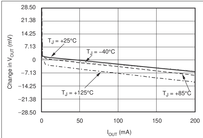
6-1. Load Regulation
