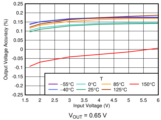
6-2. Output Accuracy vs V_{IN}
