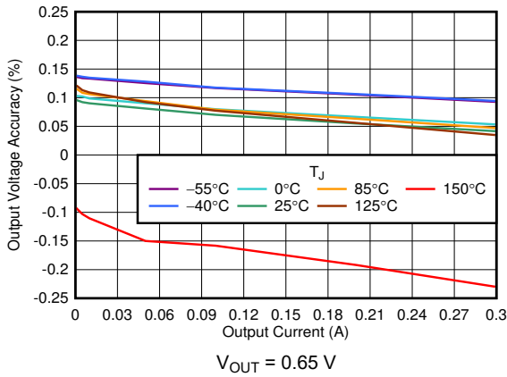
6-1. Output Accuracy vs I_{OUT}
