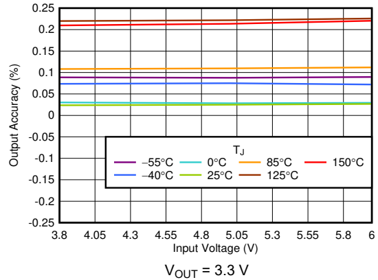
6-4. Output Accuracy vs V_{IN}
