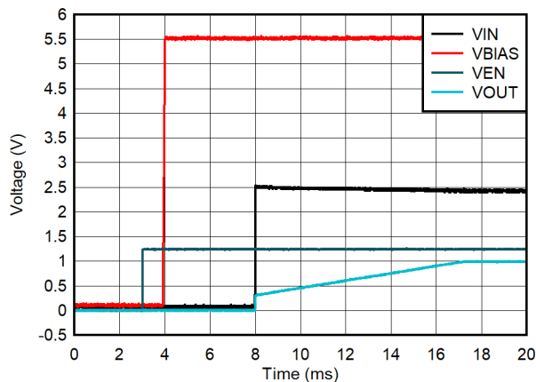
☒ 8-1. Sequencing and Soft-Start Behavior for V_{OUT} = 1\text{ V}
