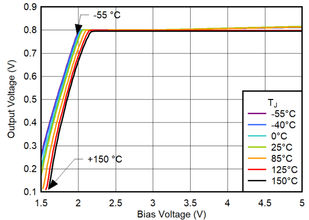
6-16. Output Voltage vs Bias Voltage
