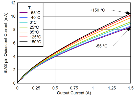
6-20. BIAS Pin Quiescent Current vs Output Current
