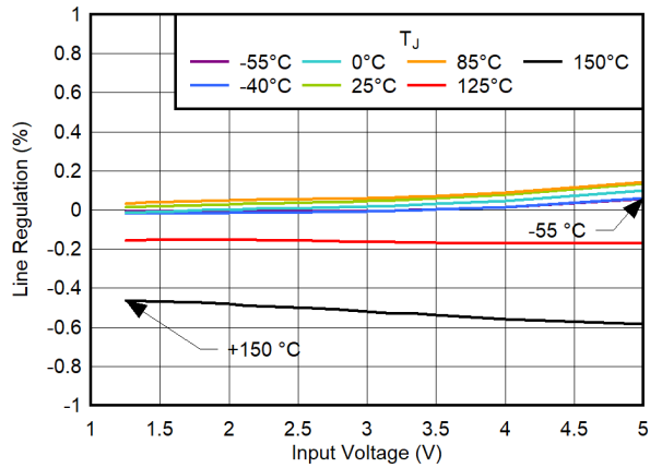
6-15. Line Regulation vs Input Voltage
