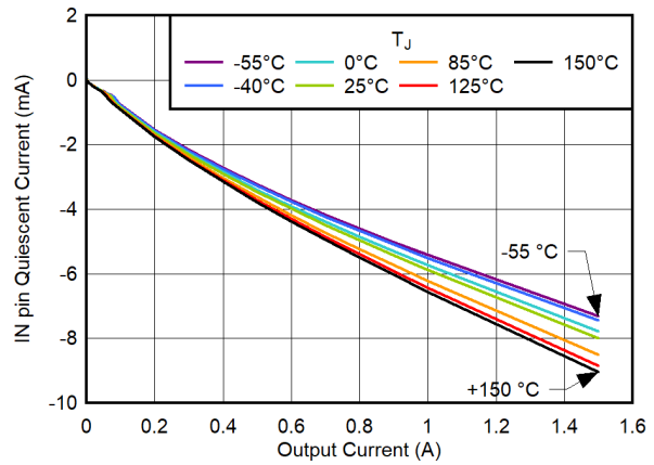
6-18. IN Pin Quiescent Current vs Output Current
