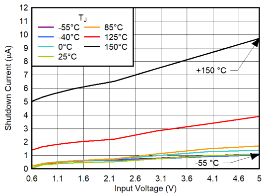
6-21. Shutdown Current (GND Pin) vs Input Voltage
