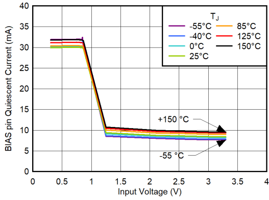
6-19. BIAS Pin Quiescent Current vs Input Voltage
