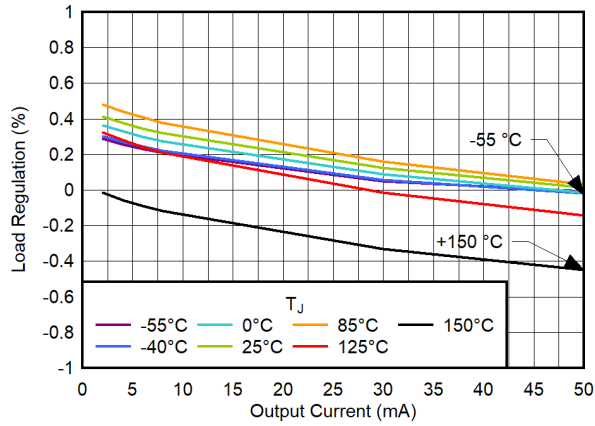
6-13. Load Regulation vs 0-mA to 50-mA Output Current
