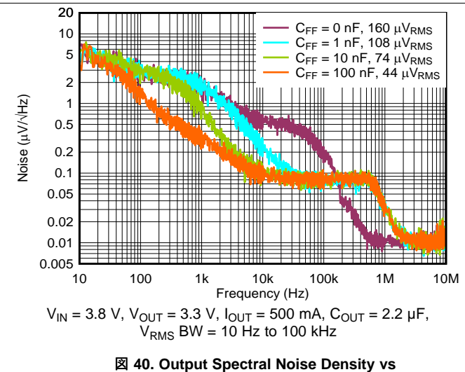
40. Output Spectral Noise Density vs Frequency and C_{FF}
