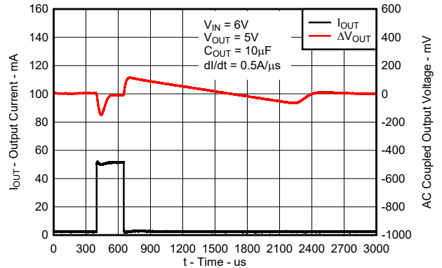
8-9. Load Transient Response for New Chip
