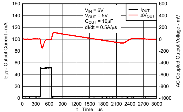
8-9. Load Transient Response for New Chip
