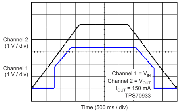
6-34. Power-Up and Power-Down Response
