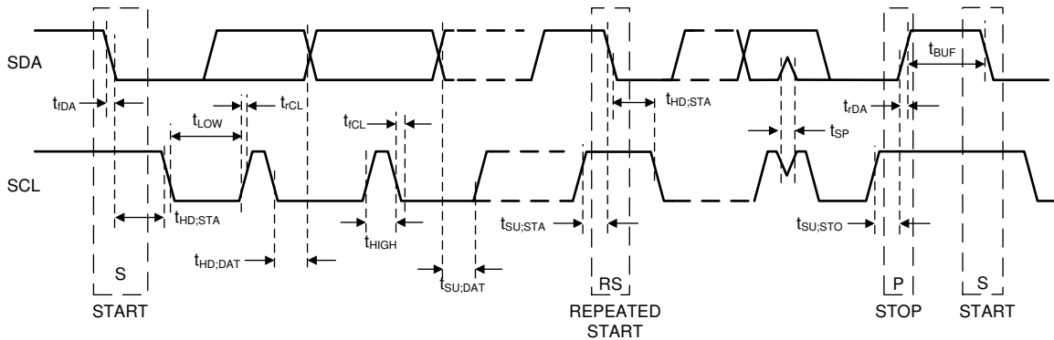
✎ 8-55. I 2 C-Compatible Timing
