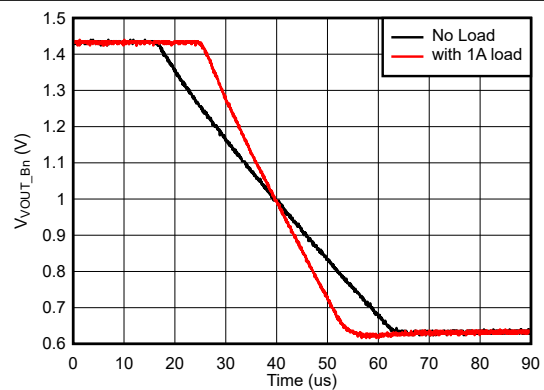
7-9. Buck Shutdown with 1A Load, Auto Mode
