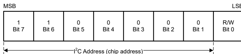
✎ 8-56. Example Device Address
