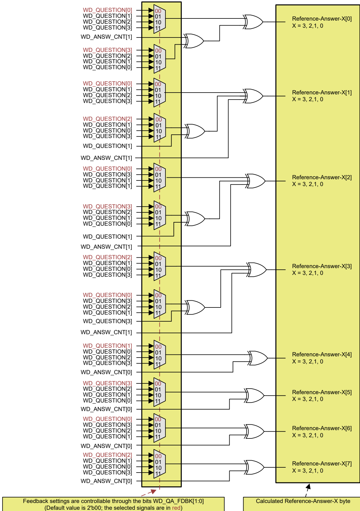
8-26. Watchdog Reference Answer Calculation
