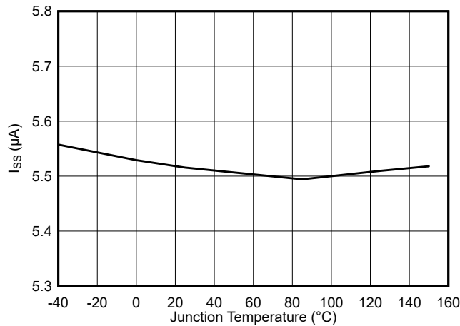
8-17. Soft-Start Charge Current vs Junction Temperature
