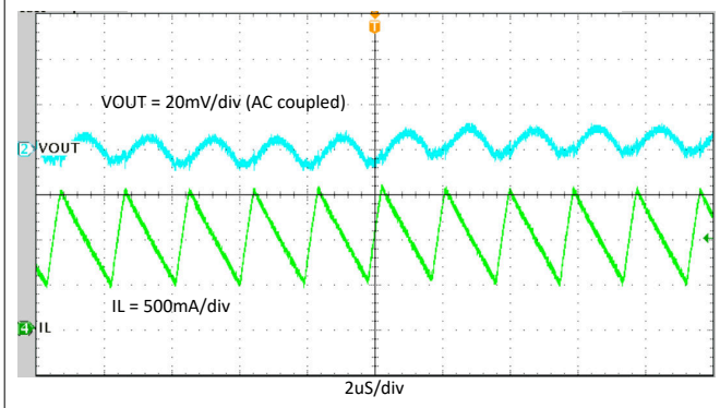
10-16. Steady State, I_{OUT} = 1 \text{ A}
