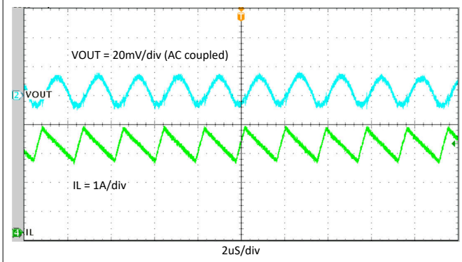
10-18. Steady State, I_{OUT} = 3 \text{ A}
