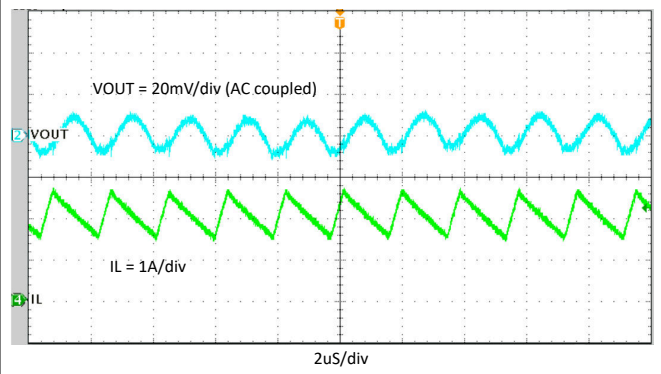
10-17. Steady State, I_{OUT} = 2 \text{ A}
