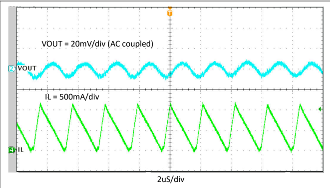
10-15. Steady State, I_{OUT} = 0.5 \text{ A}
