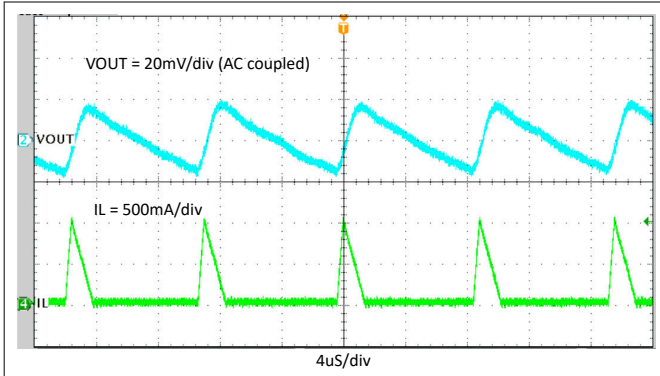
10-14. Steady State, I_{OUT} = 0.1 \text{ A}
