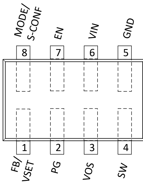
6-2. TPS629210-Q1 8-Pin DYC SOT-5X3 Pinout (TOP)
