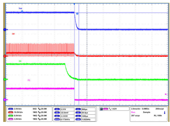
9-65. Shutdown Timing with Output Discharge Enabled
