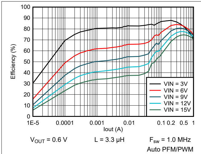
Figure 9-56. Efficiency vs Output Current
