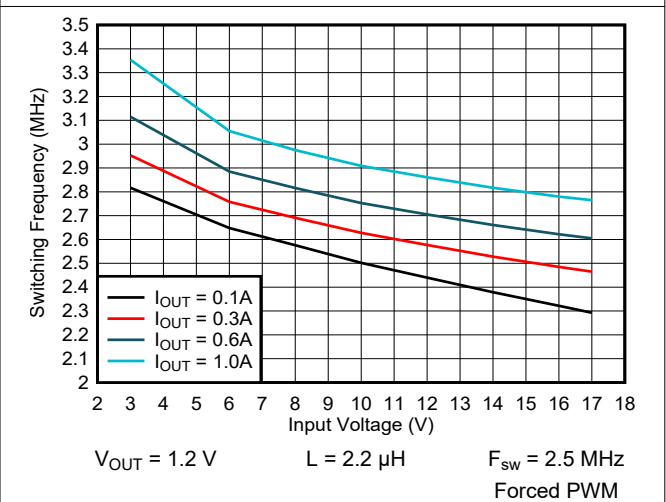
9-41. Switching Frequency vs Input Voltage
