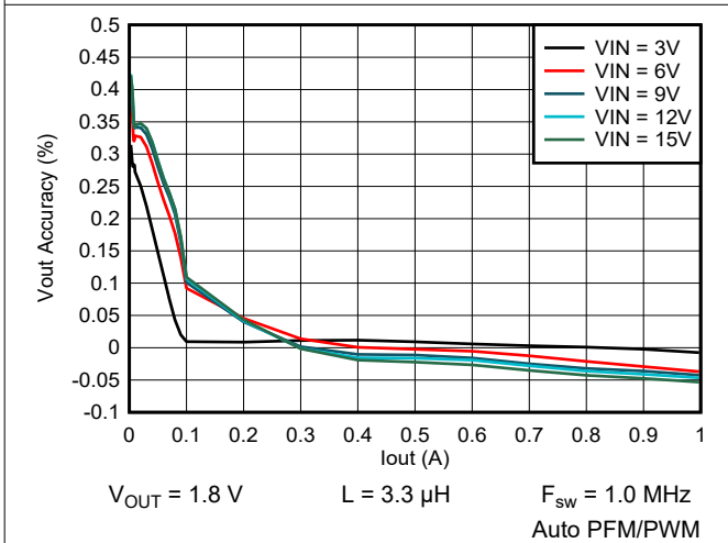
9-36. Output Voltage vs Output Current
