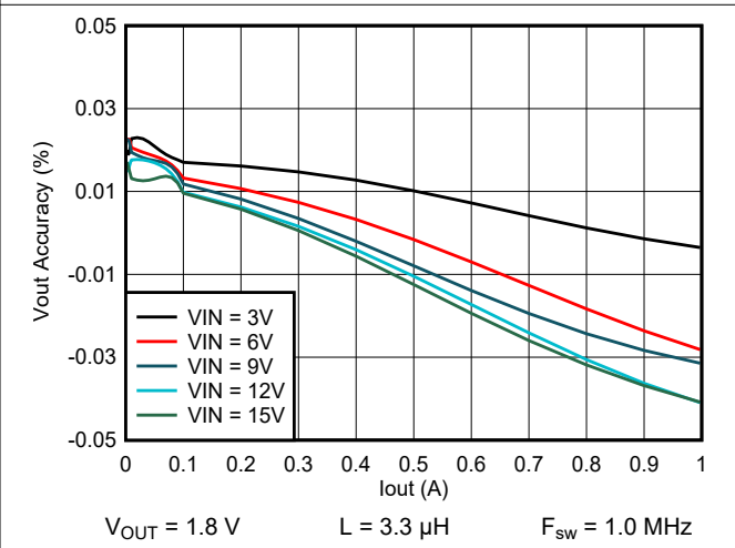
9-37. Output Voltage vs Output Current
