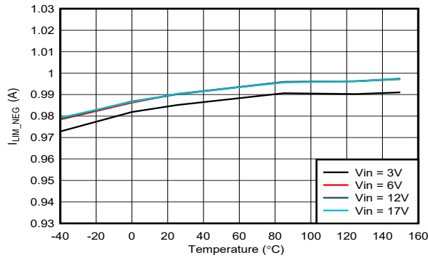
7-15. Low-Side I_{NEG} vs Temperature
