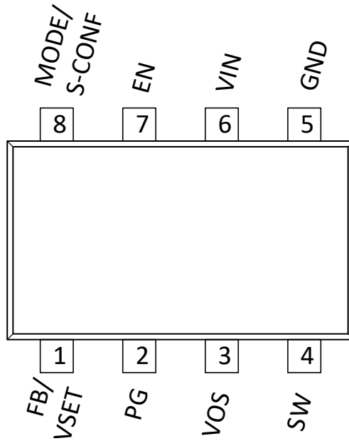
6-1. TPS629210-Q1 8-Pin DRL SOT-5X3 Pinout (TOP)
