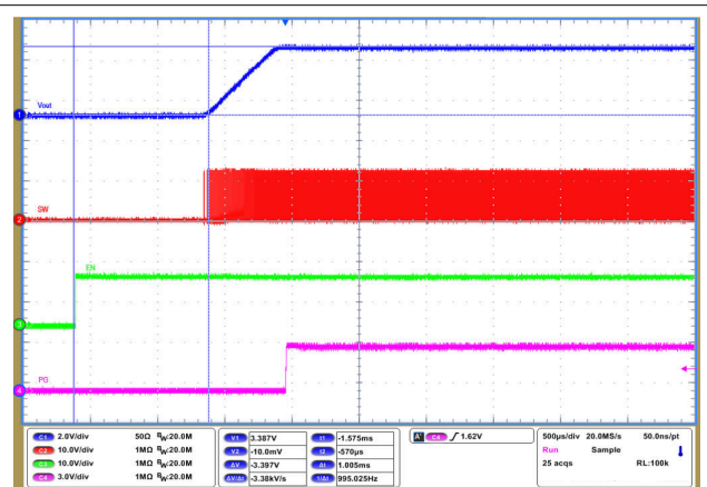
9-63. Start-Up Timing
