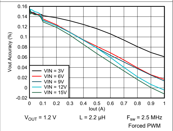
9-43. Output Voltage vs Output Current
