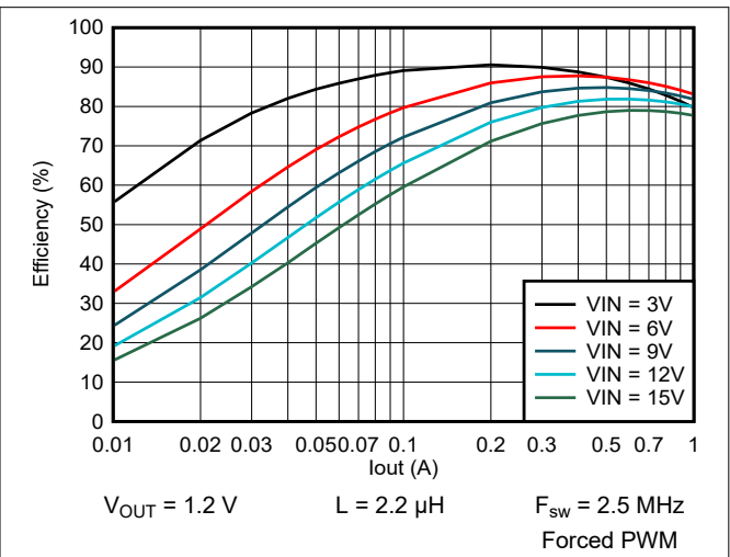
9-39. Efficiency vs Output Current
