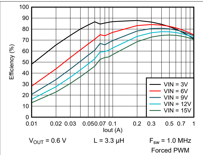
Figure 9-57. Efficiency vs Output Current
