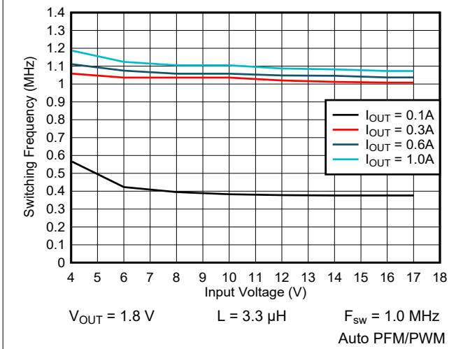
9-34. Switching Frequency vs Input Voltage
