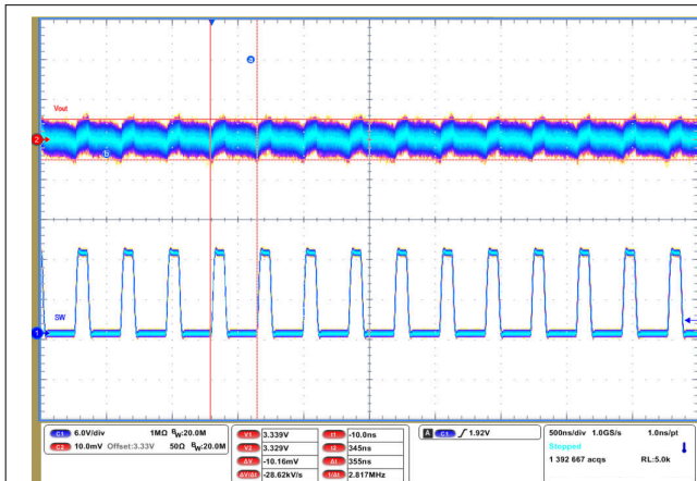
9-74. Output Voltage Ripple
