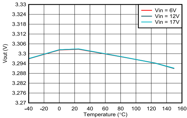
7-3. Output Voltage Accuracy – External Feedback
