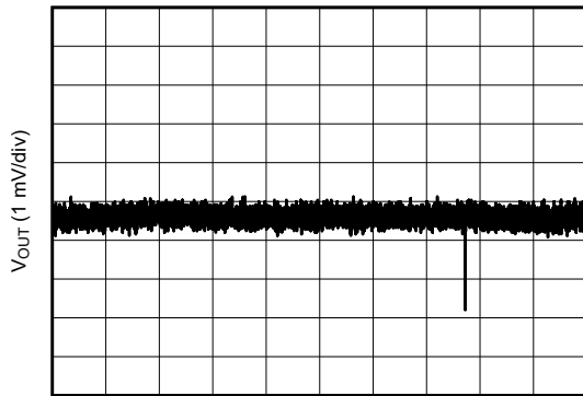
12 V to 1.8 V, 2 A 1 \mu\text{H} , 1.4 MHz First and second L-C
