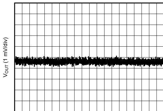
12 V to 3.3 V, 2 A 1 \mu\text{H} , 2.2 MHz First and second L-C
