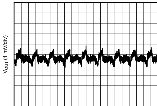
12 V to 3.3 V, 2 A 1 \mu\text{H} , 2.2 MHz First L-C Only
