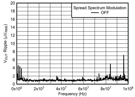
12 V to 1.8 V, 2 A 1 \mu\text{H} , 1.4 MHz First and second L-C BW = 10 kHz
