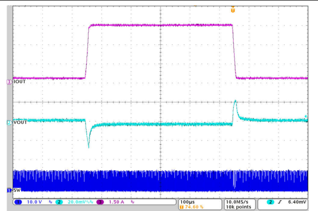
7-12. Load Transient
