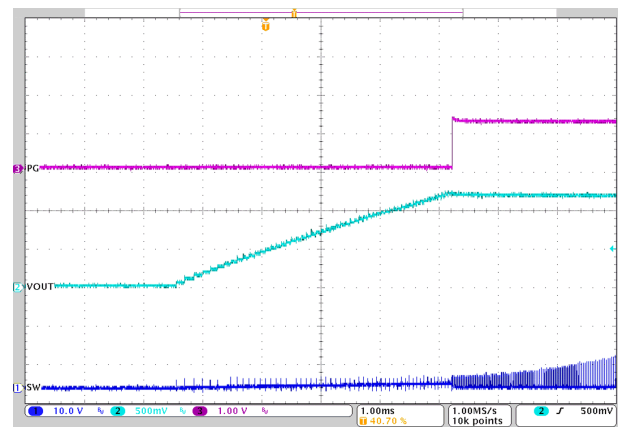
7-10. Start-up
