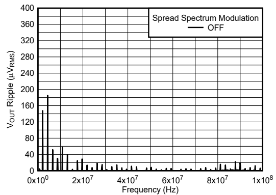
12 V to 3.3 V, 2 A 1 \mu\text{H} , 2.2 MHz First L-C Only BW = 10 kHz
