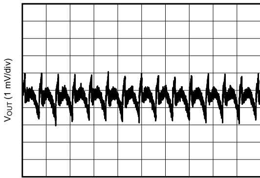
図 5-3. V_{OUT} Ripple After the Second L-C Filter
