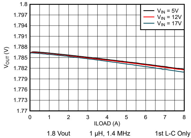
7-8. Output Voltage vs Load Current
