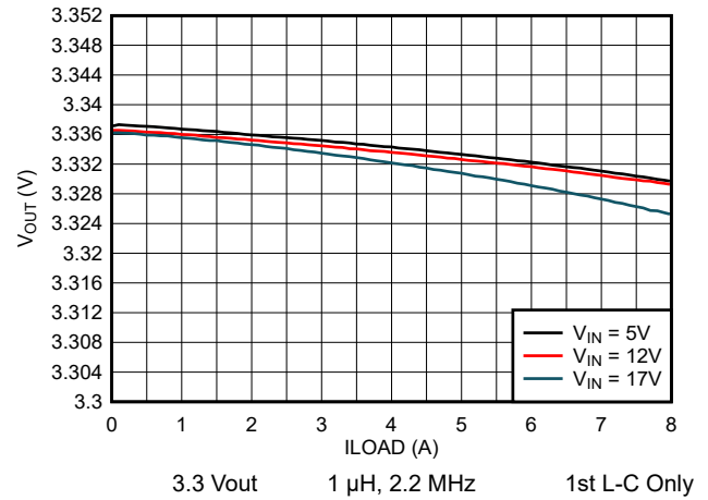
7-9. Output Voltage vs Load Current
