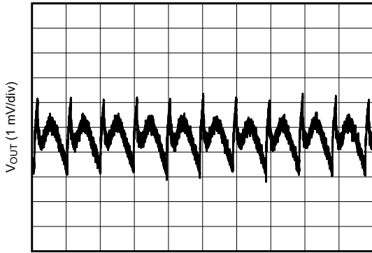
図 5-1. V_{OUT} Ripple After the First L-C Filter
