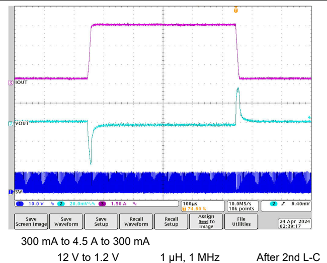
7-13. Load Transient
