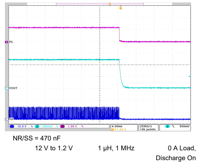
7-11. Shutdown
