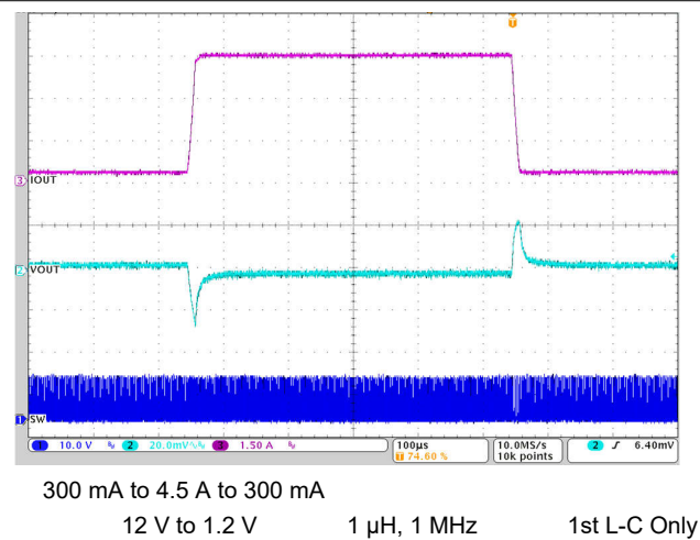
7-12. Load Transient
