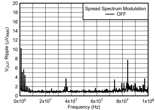
図 5-2. V_{OUT} Ripple FFT After the First L-C Filter
