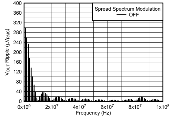
図 5-2. V_{OUT} Ripple FFT After the First L-C Filter
