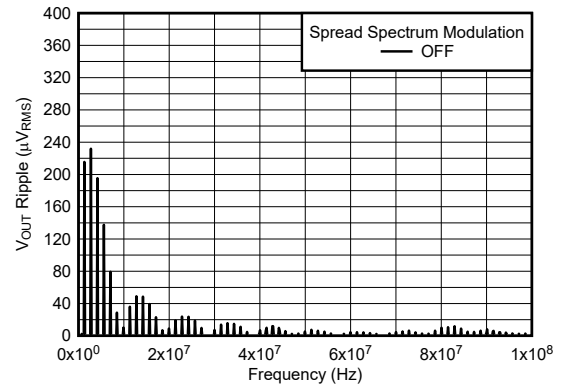
図 5-4. V_{OUT} Ripple FFT After the Second L-C Filter
