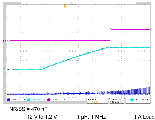
7-10. Start-up
