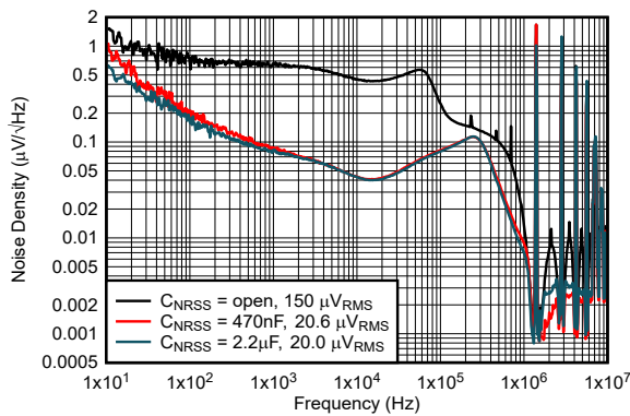
5-13. Output Noise Density vs Frequency
