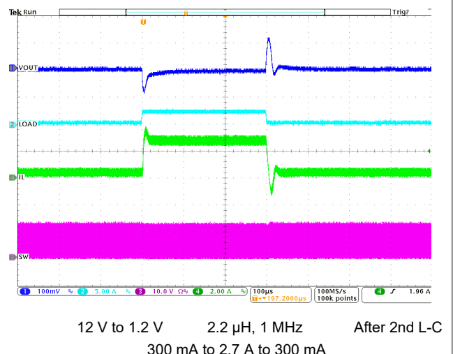
8-13. Load Transient
