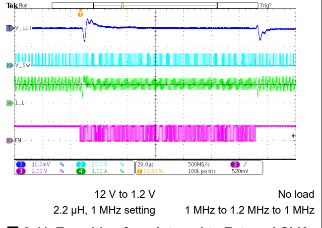
8-11. Transition from Internal to External CLK
