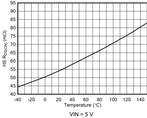
Fig 6-49. High-Side R_{DS(ON)} vs Junction Temperature
