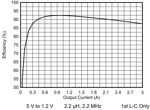
8-8. Efficiency vs Load Current
