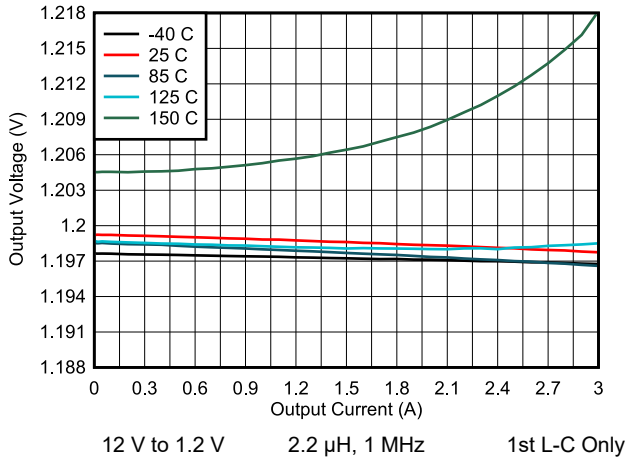
8-10. Output Voltage vs Load Current
