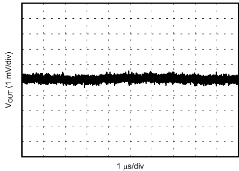
6-7. V_{OUT} Ripple After the First L-C Filter
