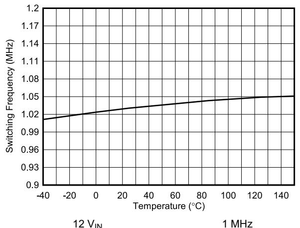
Fig 6-54. Oscillator Frequency vs Temperature
