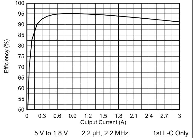
8-9. Efficiency vs Load Current
