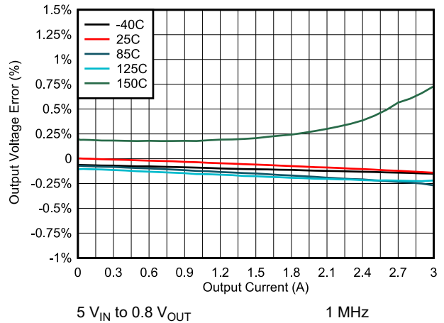
Fig 6-52. Output Voltage Error vs Load
