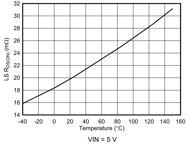
Fig 6-50. Low-Side R_{DS(ON)} vs Junction Temperature
