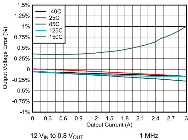
Fig 6-53. Output Voltage Error vs Load
