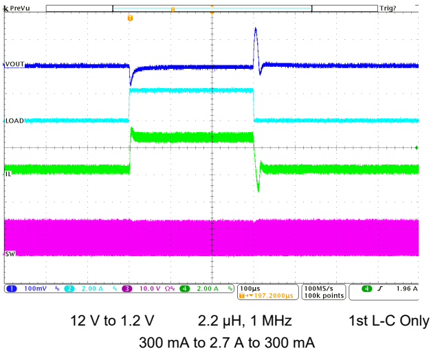
8-12. Load Transient
