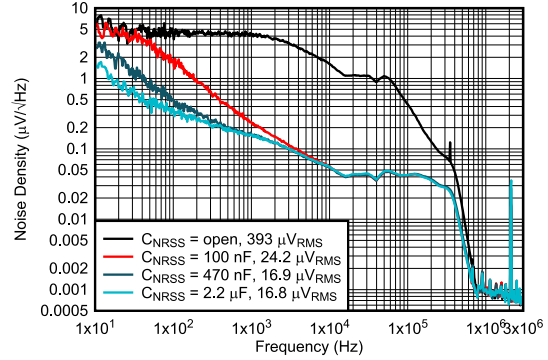
6-38. Output Noise Density vs Frequency
