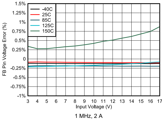
Fig 6-51. FB Pin Voltage Error vs Input Voltage
