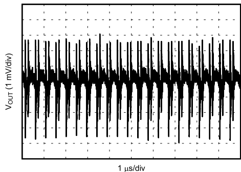
6-9. V_{OUT} Ripple After the Second L-C Filter
