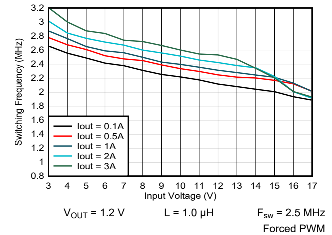
9-18. Switching Frequency vs Input Voltage
