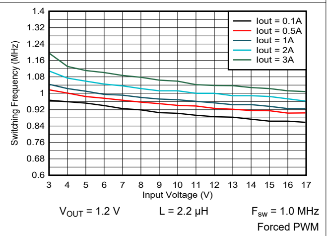
9-24. Switching Frequency vs Input Voltage
