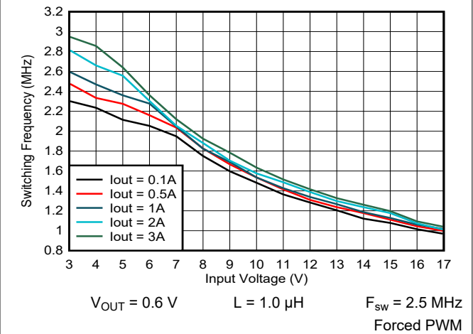
9-30. Switching Frequency vs Input Voltage
