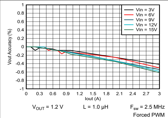
9-20. Output Voltage vs Output Current
