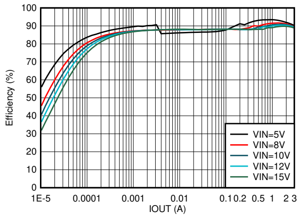
Figure 8-11. Efficiency vs Output Current V OUT = 3.3 V
