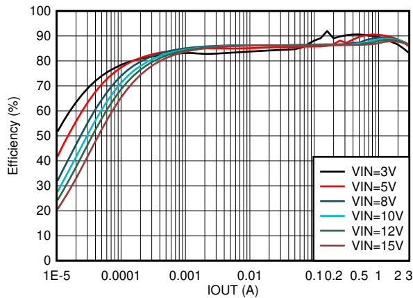
Figure 8-13. Efficiency vs Output Current V OUT = 1.8 V
