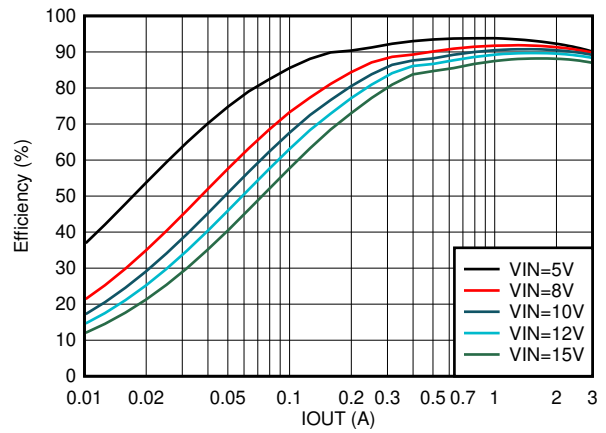
Figure 8-12. Efficiency vs Output Current V OUT = 3.3 V
