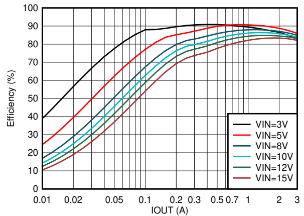
Figure 8-14. Efficiency vs Output Current V OUT = 1.8 V
