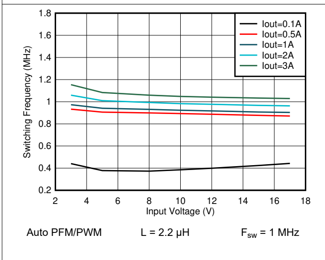
Figure 8-33. Switching Frequency vs Input Voltage V OUT = 1.2 V
