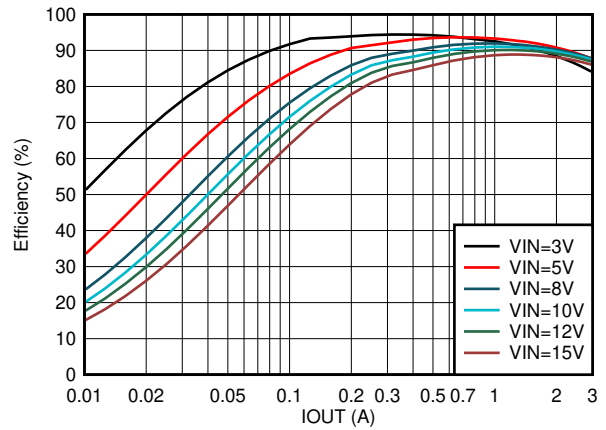
Figure 8-12. Efficiency vs Output Current V OUT = 3.3 V
