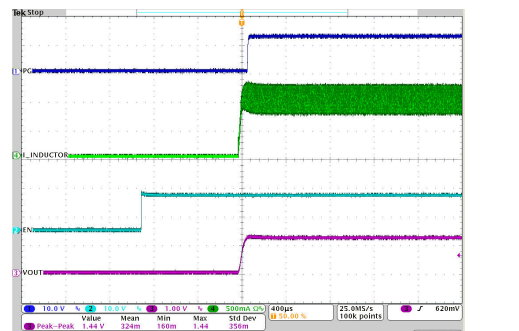
V_{IN} = 12 V 1 MHz Auto PFM/PWM I_o = 1 A V_{OUT} = 1.2 V T_A = 25^\circ\text{C}
