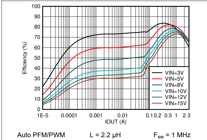
Figure 8-68. Efficiency vs Output Current V_{OUT} = 0.4\text{ V}
