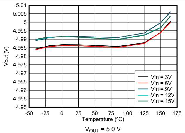
Figure 7-4. Output Voltage Accuracy - VSET Selected V_{OUT} = 5.0\text{ V}
