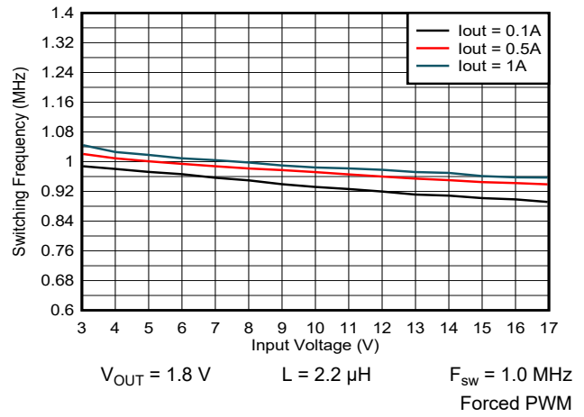
9-12. Switching Frequency vs Input Voltage
