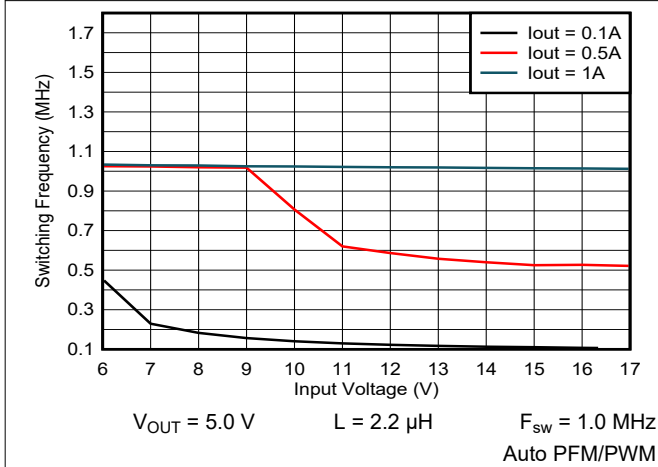
图 9-48. Switching Frequency vs Input Voltage
