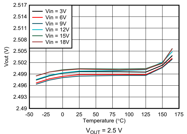
Figure 7-6. Output Voltage Accuracy - VSET Selected V_{OUT} = 2.5\text{ V}
