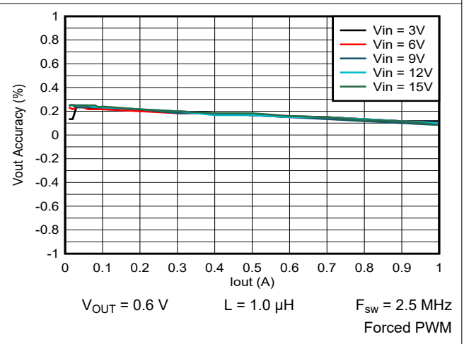
9-32. Output Voltage vs Output Current
