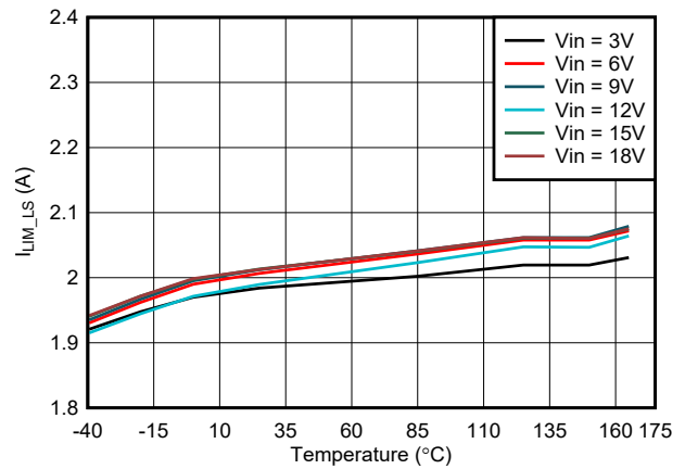
图 7-16. Low Side I_{LIM} vs Temperature
