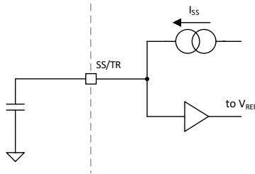
图 9-2. Soft-Start Operation Simplified Schematic
