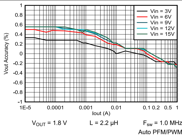
9-13. Output Voltage vs Output Current
