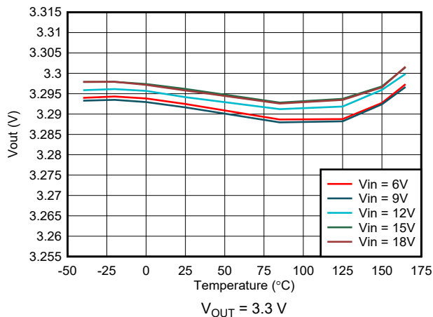
Figure 7-5. Output Voltage Accuracy - VSET Selected V_{OUT} = 3.3\text{ V}
