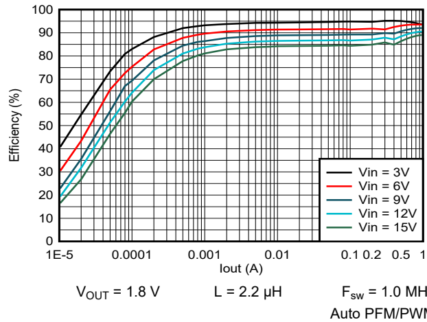
9-9. Efficiency vs Output Current
