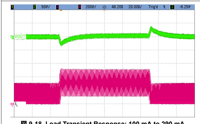
图 9-18. Load Transient Response; 100 mA to 290 mA
