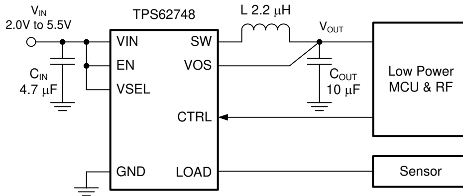
図 9-1. TPS62748 Typical Application Circuit
