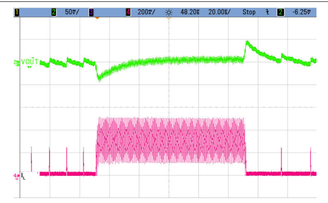
图 9-19. Load Transient Response; 5 mA to 290 mA
