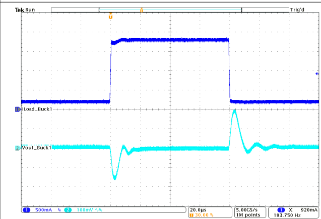
10-29. Load Transient Response
