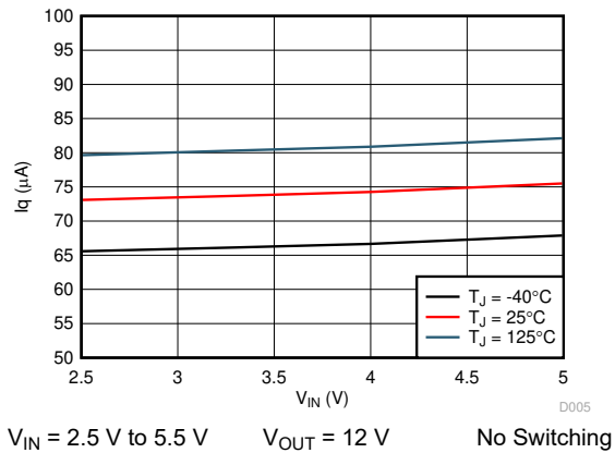
6-5. I_q vs V_{IN}
