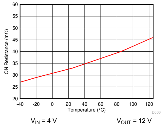
6-6. Low-Side R_{DS(ON)} vs Temperature
