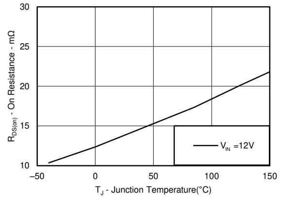
5-4. High-side R DS(on) vs Temperature
