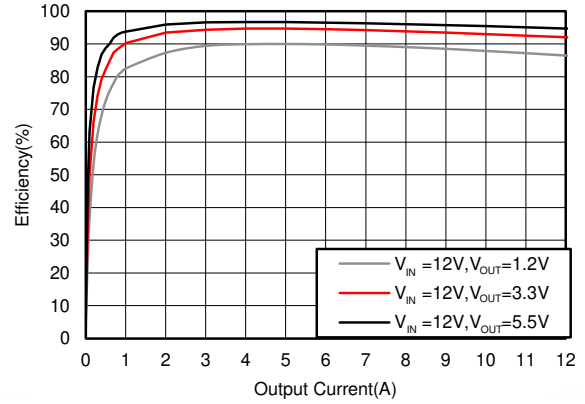
5-14. Efficiency, Mode = FCCM, F_{SW} = 400 kHz
