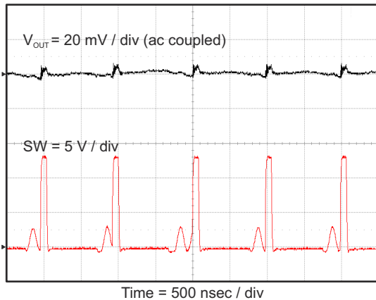
図 7-12. Output Voltage Ripple, I_{OUT} = 800 \text{ mA}
