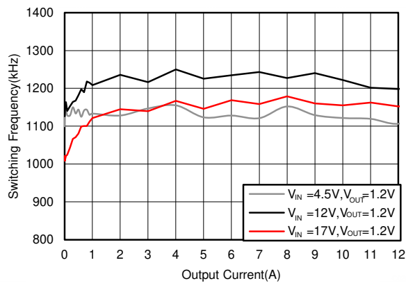
5-23. F_{SW} Load Regulation, Mode = FCCM, F_{SW} = 1200 kHz
