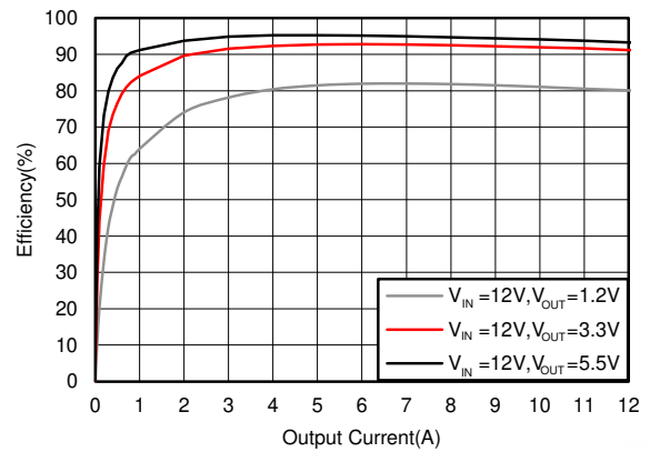
5-16. Efficiency, Mode = FCCM, F_{SW} = 1200 kHz
