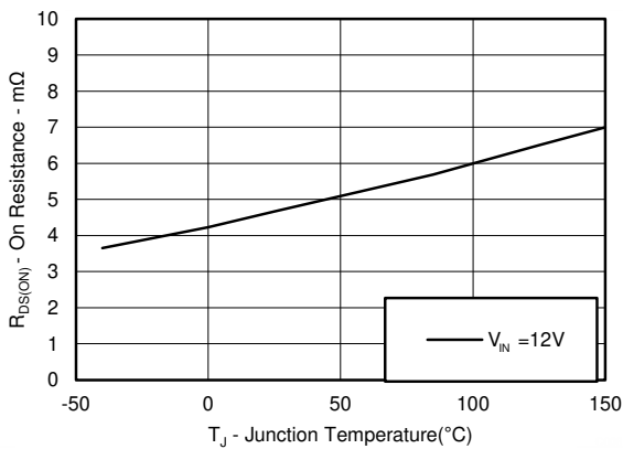
5-5. Low-side R DS(on) vs Temperature
