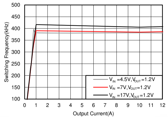
5-18. F_{SW} Load Regulation, Mode = DCM, F_{SW} = 400 kHz
