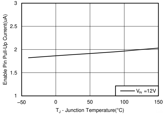
5-7. Enable Pullup Current, V_{EN} = 1.0\text{ V}
