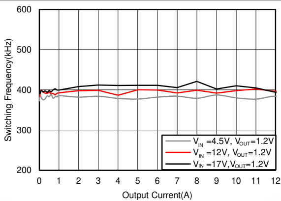
5-21. F_{SW} Load Regulation, Mode = FCCM, F_{SW} = 400 kHz
