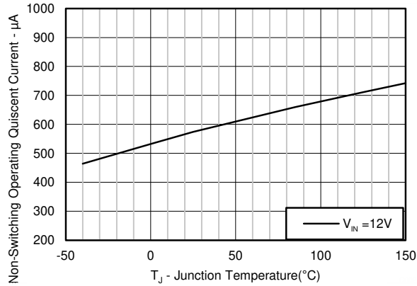
5-1. Quiescent Current vs Temperature
