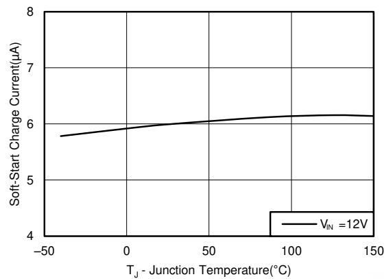
5-6. Soft-Start Charge Current vs Temperature
