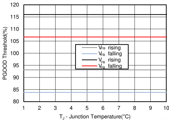
5-9. PGOOD Threshold vs Temperature
