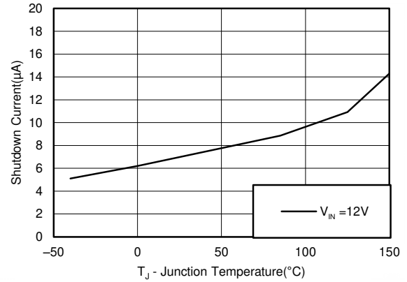
5-2. Shutdown Current vs Temperature
