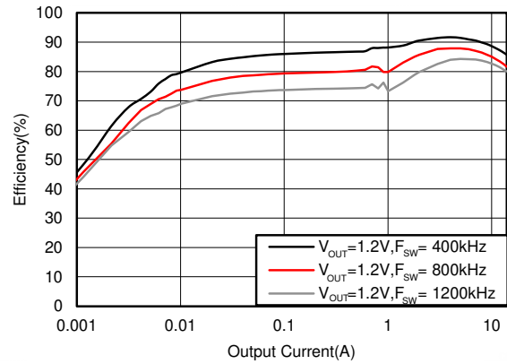
5-12. Efficiency with External VREG5 = 5 V, V_{IN} = 12\text{ V}
