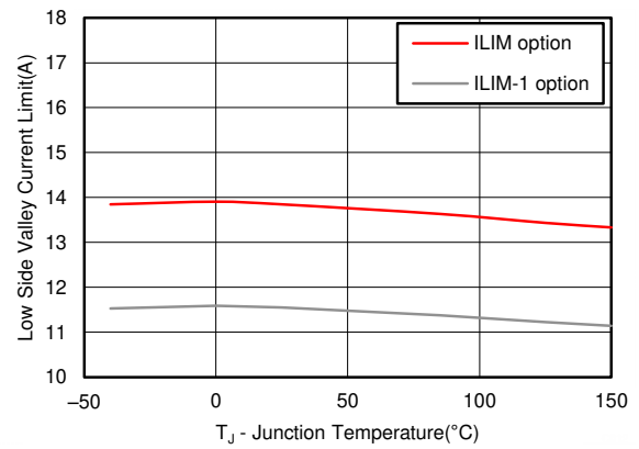
5-10. Current Limit vs Temperature
