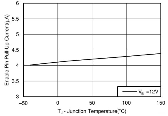
5-8. Enable Pullup Current, V_{EN} = 1.3\text{ V}
