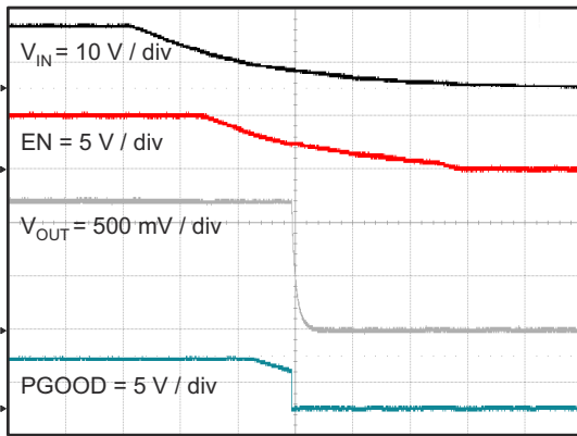
図 7-16. Shut Down Relative to V_{IN} Falling
