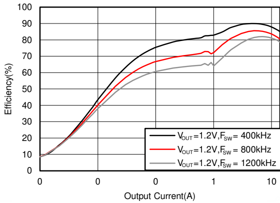
5-11. Efficiency with Internal VREG5 = 4.7 V, V_{IN} = 12\text{ V}
