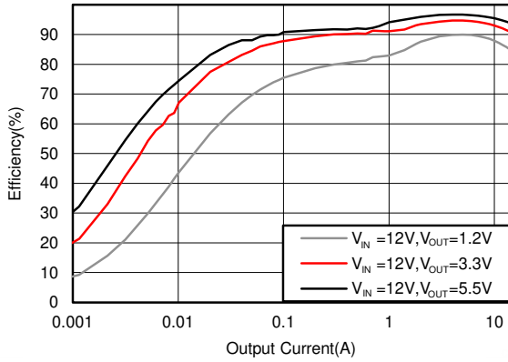
5-13. Efficiency, Mode = DCM, F_{SW} = 400 kHz
