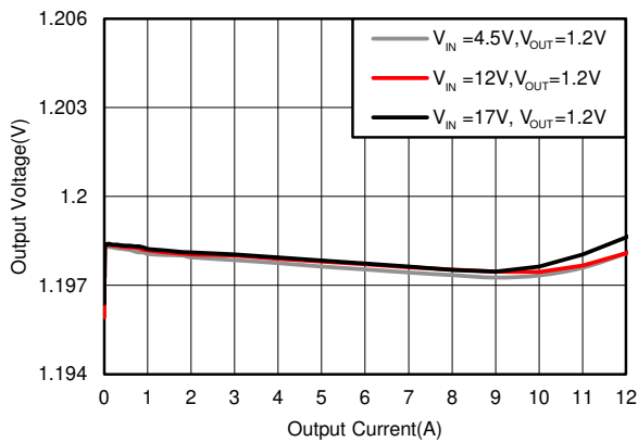
5-17. Load Regulation, F_{SW} = 800 kHz
