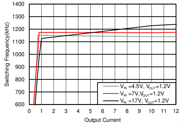
5-20. F_{SW} Load Regulation, Mode = DCM, F_{SW} = 1200 kHz
