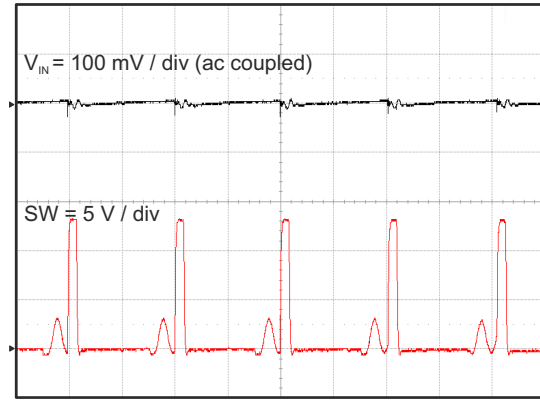
図 7-9. Input Voltage Ripple, I_{OUT} = 800 \text{ mA}
