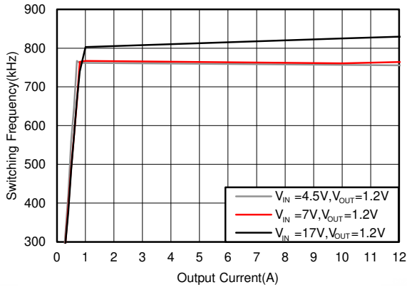
5-19. F_{SW} Load Regulation, Mode = DCM, F_{SW} = 800 kHz
