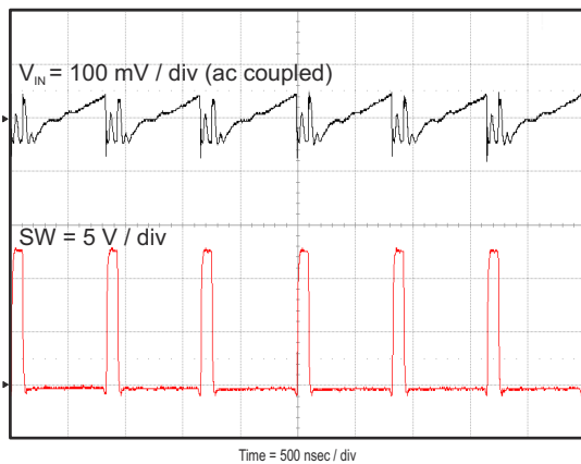
図 7-10. Input Voltage Ripple, I_{OUT} = 12 \text{ A}
