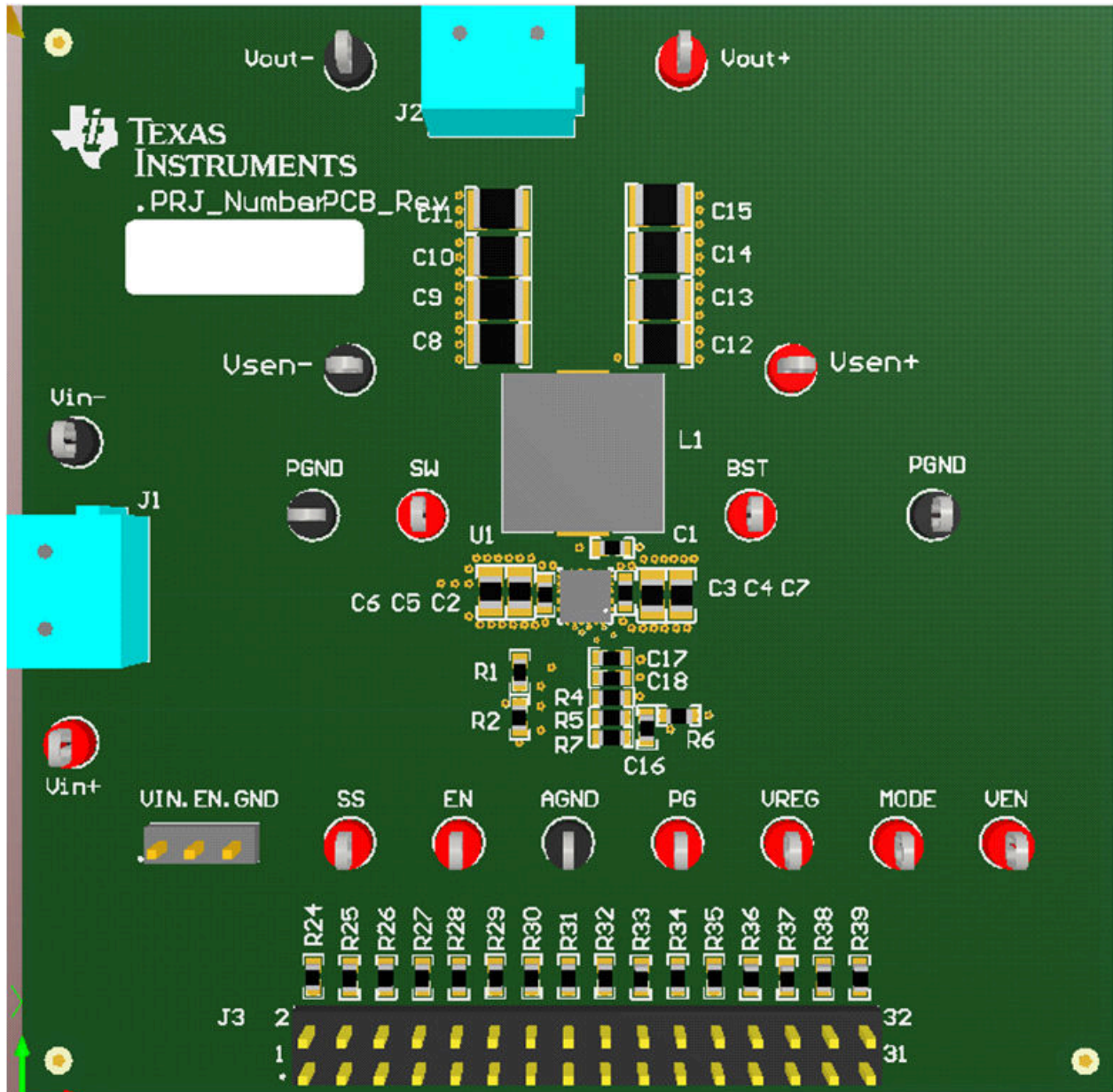
図 8-1. System Validation EVM Board
