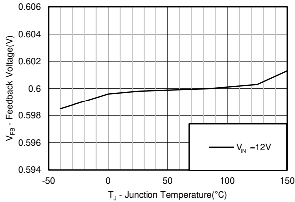
5-3. Feedback Voltage vs Temperature
