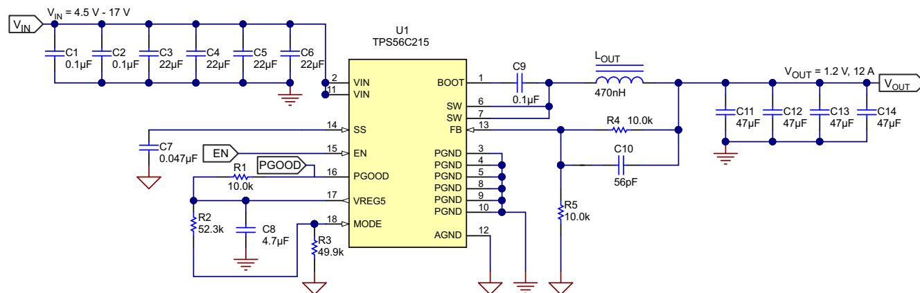
図 7-1. Application Schematic
