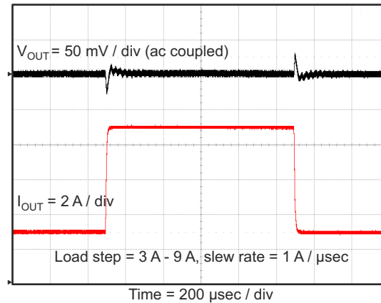
図 7-18. Transient Response
