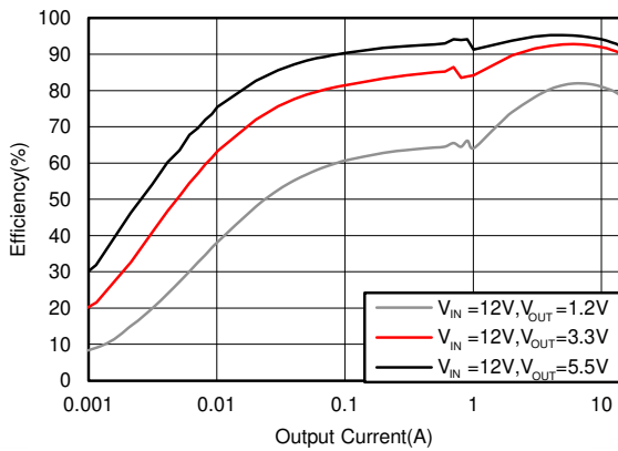
5-15. Efficiency, Mode = DCM, F_{SW} = 1200 kHz
