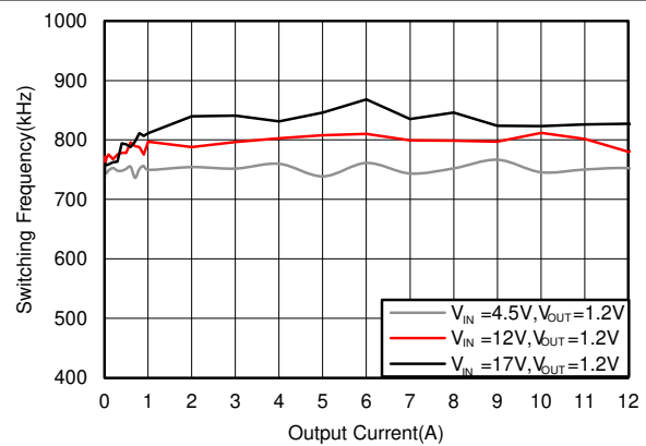
5-22. F_{SW} Load Regulation, Mode = FCCM, F_{SW} = 800 kHz
