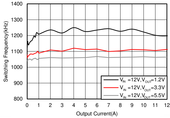
5-25. F_{SW} Load Regulation, Mode = FCCM, F_{SW} = 1200 kHz
