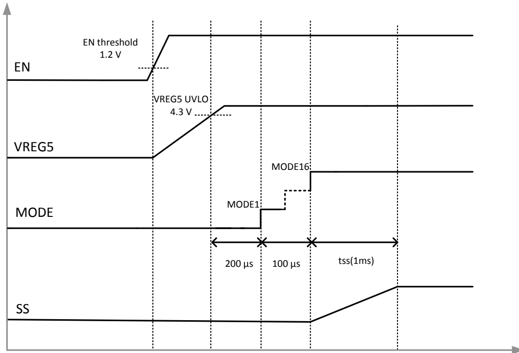
図 6-2. Power-Up Sequence
