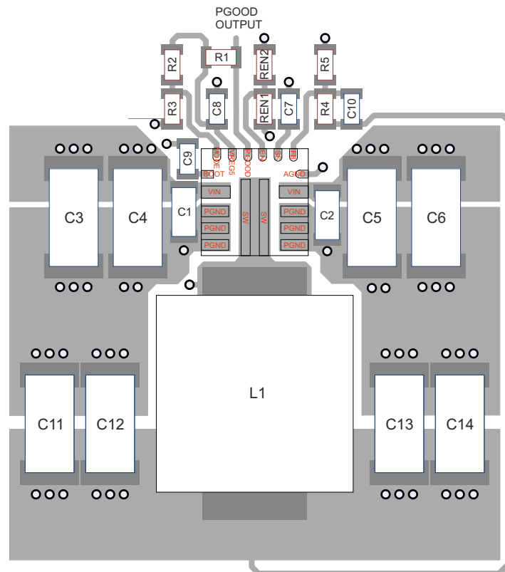
☒ 7-19. Top Side Layout
