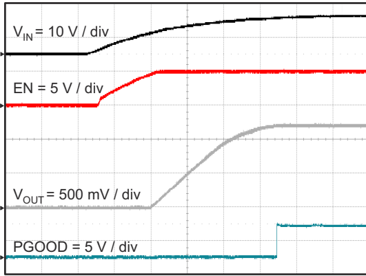
図 7-14. Start Up Relative to V_{IN} Rising
