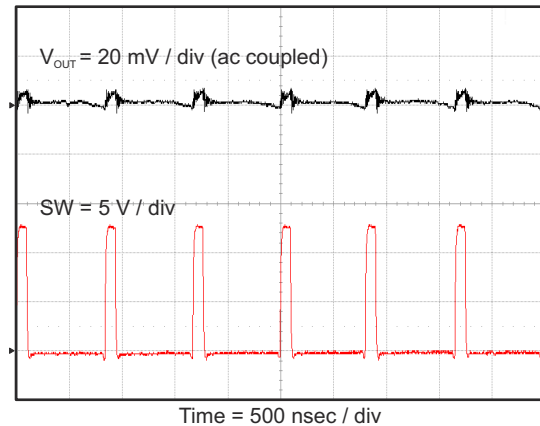
図 7-13. Output Voltage Ripple, I_{OUT} = 12 \text{ A}
