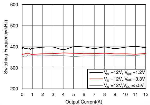
5-24. F_{SW} Load Regulation, Mode = FCCM, F_{SW} = 400 kHz
