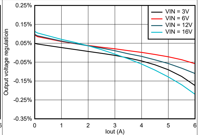
8-5. TPS566247 Load Regulation vs Loading
