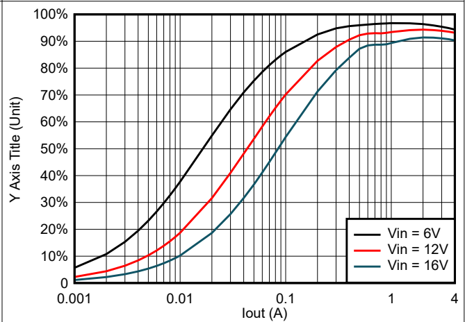
6-16. TPS564247 Efficiency at 3.3 V_{OUT} with a 1.5\text{-}\mu\text{H} Inductor
