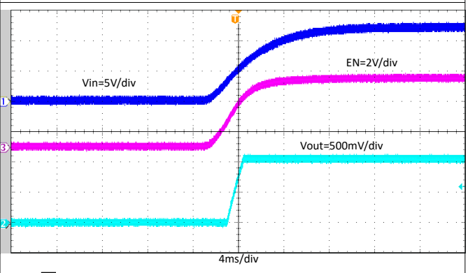
图 8-13. Start-Up with V_{IN} Rising, I_{OUT} = 4\text{ A}
