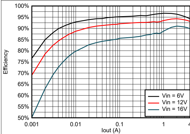
6-15. TPS564242 Efficiency at 3.3 V_{OUT} with a 1.5\text{-}\mu\text{H} Inductor
