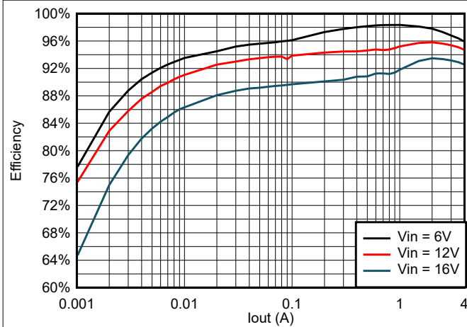
6-17. TPS564242 Efficiency at 5 V_{OUT} with a 1.8\text{-}\mu\text{H} Inductor
