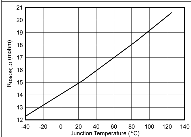
图 6-5. Low-Side R_{DS(ON)}
