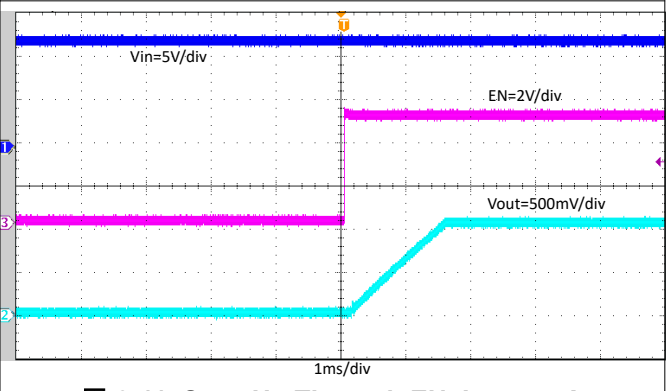
图 8-11. Start-Up Through EN, I_{OUT} = 4\text{ A}
