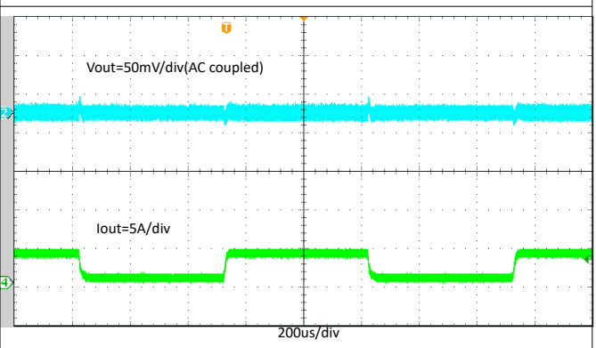
图 8-15. TPS564242 Transient Response with 0.4 A to 3.6 A by 2.5-A/ \mu\text{s} Load Step
