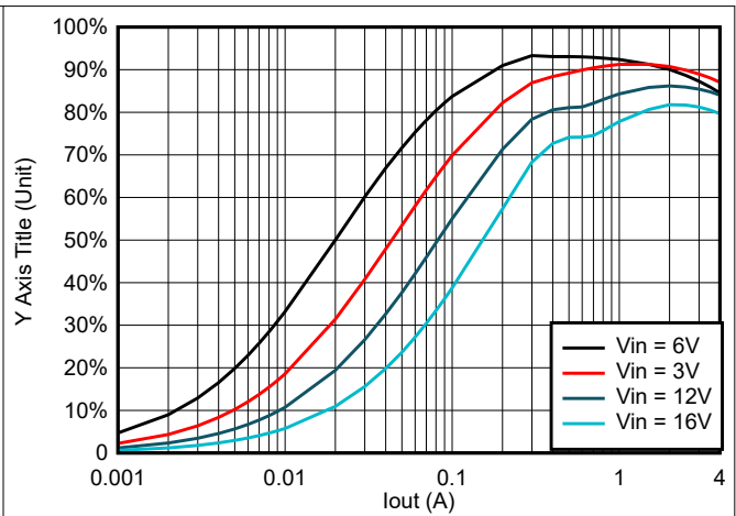
6-14. TPS564247 Efficiency at 1.05 V_{OUT} with a 0.82\text{-}\mu\text{H} Inductor
