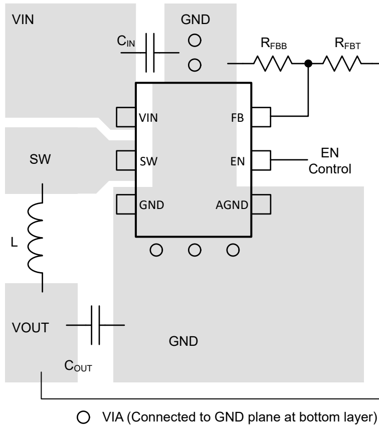
☒ 10-1. Suggested Layout
