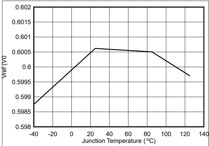
Figure 6-7. V_{REF} Voltage
