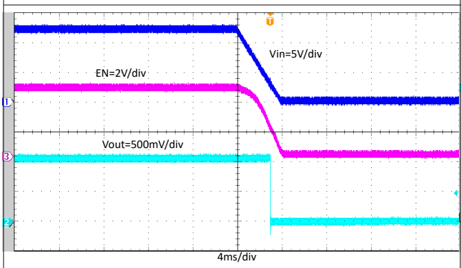
图 8-14. Start-Up with V_{IN} Falling, I_{OUT} = 4\text{ A}
