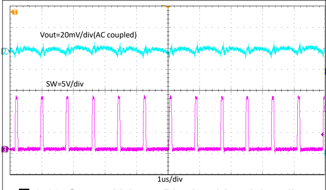
图 8-10. Output Voltage Ripple with 4-A Loading
