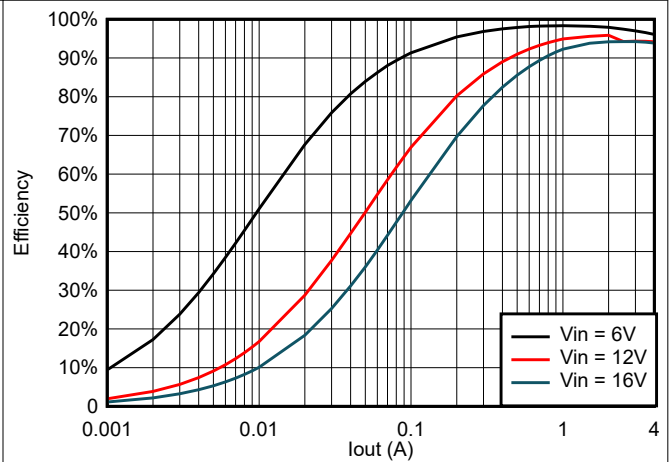
6-18. TPS564247 Efficiency at 5 V_{OUT} with a 1.8\text{-}\mu\text{H} Inductor
