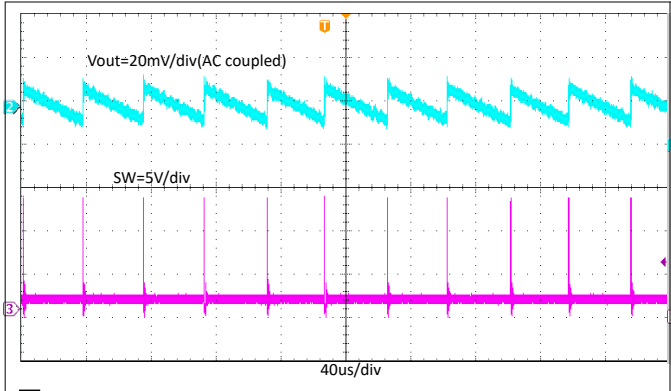
图 8-8. TPS564242 Output Voltage Ripple with 0.01-A Loading
