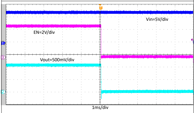
图 8-12. Shutdown Through EN, I_{OUT} = 4\text{ A}
