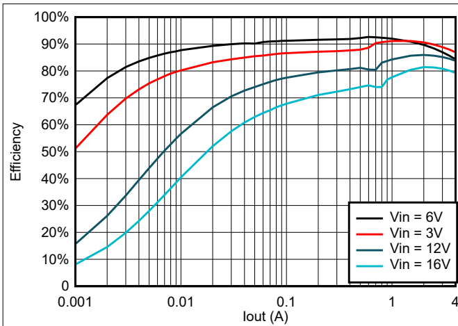
6-13. TPS564242 Efficiency at 1.05 V_{OUT} with a 0.82\text{-}\mu\text{H} Inductor
