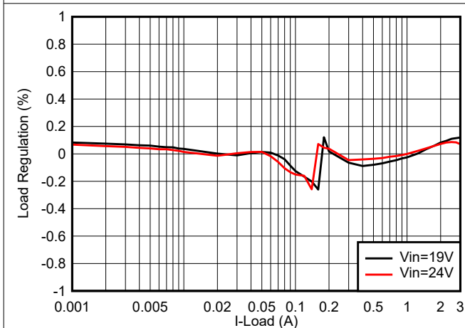
6-17. Load Regulation, V_{OUT} = 12\text{ V} , f_{SW} = 500\text{ kHz}
