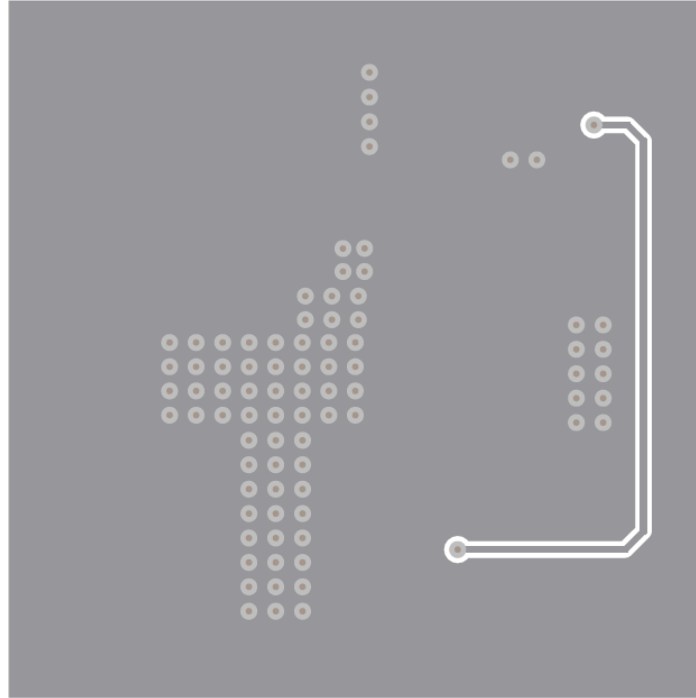
☒ 8-24. TPS563300 Bottom Layout Example
