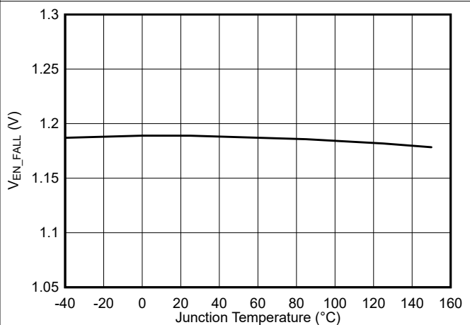
6-6. Disable Threshold vs Junction Temperature
