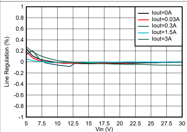
6-18. Line Regulation, V_{OUT} = 3.3\text{ V} , f_{SW} = 500\text{ kHz}
