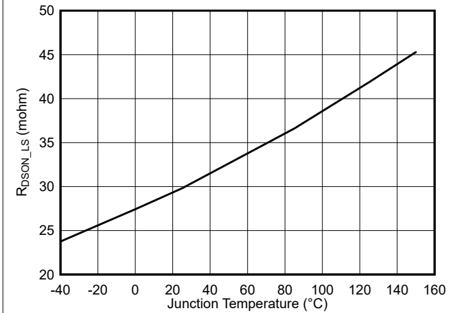
6-3. Low-Side R_{DS(on)} vs Junction Temperature
