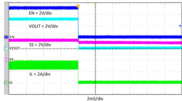
8-11. Shutdown Through EN, I_{OUT} = 3\text{ A}
