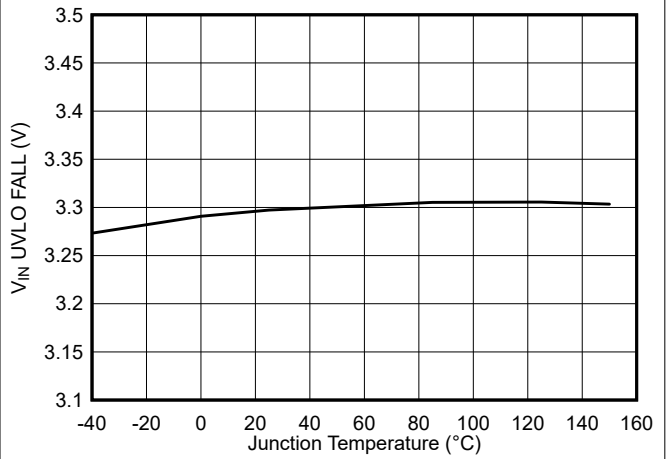
6-8. V IN UVLO Falling Threshold vs Junction Temperature
