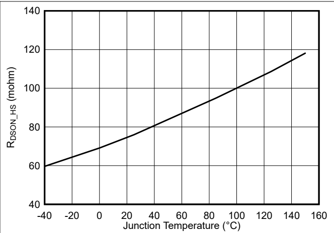
6-2. High-Side R_{DS(on)} vs Junction Temperature
