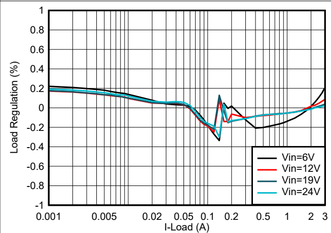
6-16. Load Regulation, V_{OUT} = 3.3\text{ V} , f_{SW} = 500\text{ kHz}
