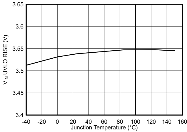
6-7. V IN UVLO Rising Threshold vs Junction Temperature
