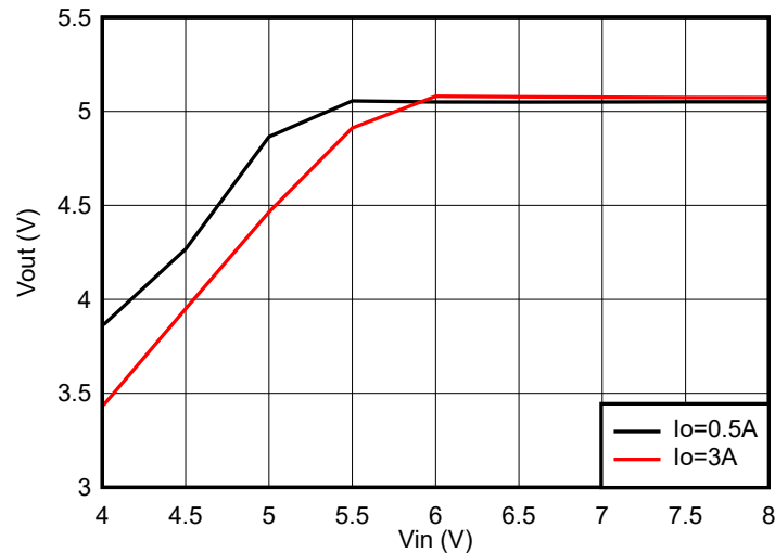
☒ 7-6. Overall Dropout Characteristic, V OUT = 5 V
