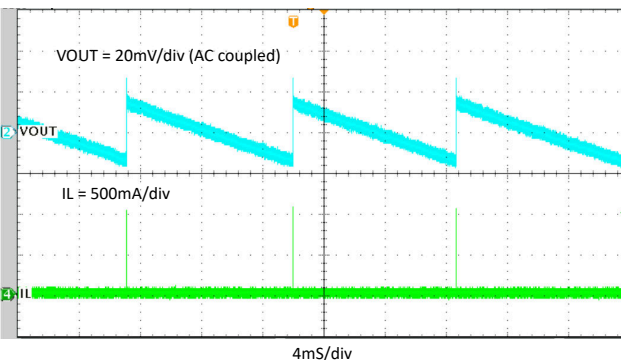
8-12. Steady State, I_{OUT} = 0\text{ A}
