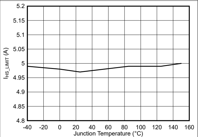
6-10. High-Side Current Limit vs Junction Temperature
