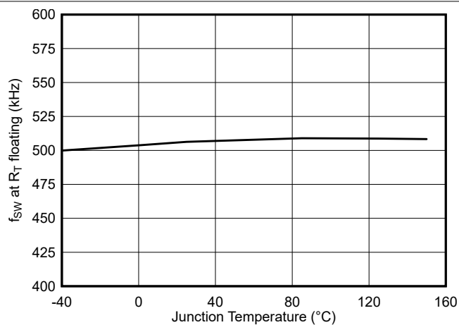
6-9. Switching Frequency vs Junction Temperature
