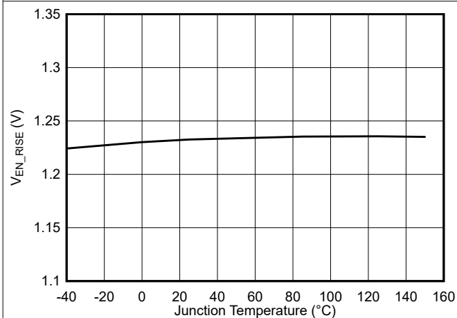
6-5. Enable Threshold vs Junction Temperature
