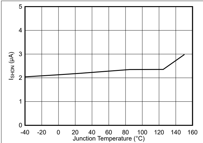
6-1. Shutdown Current vs Junction Temperature
