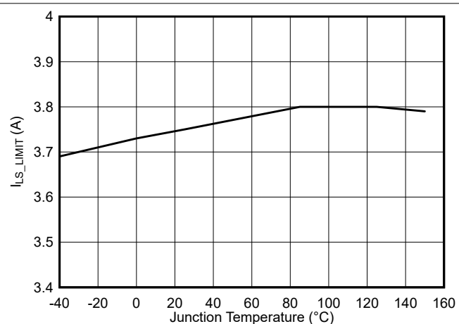
6-11. Low-Side Current Limit vs Junction Temperature
