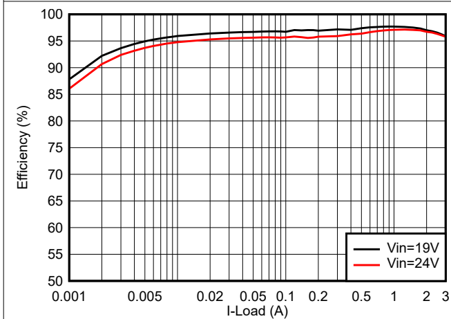
6-15. Efficiency, V_{OUT} = 12\text{ V} , f_{SW} = 500\text{ kHz} , L = 12\text{ }\mu\text{H}
