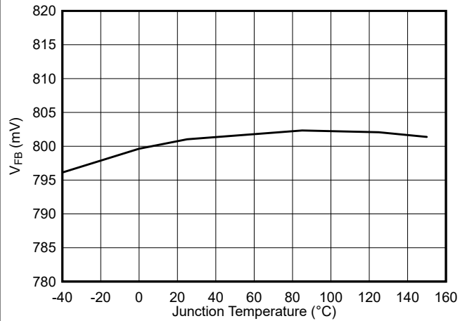
6-4. Feedback Voltage vs Junction Temperature
