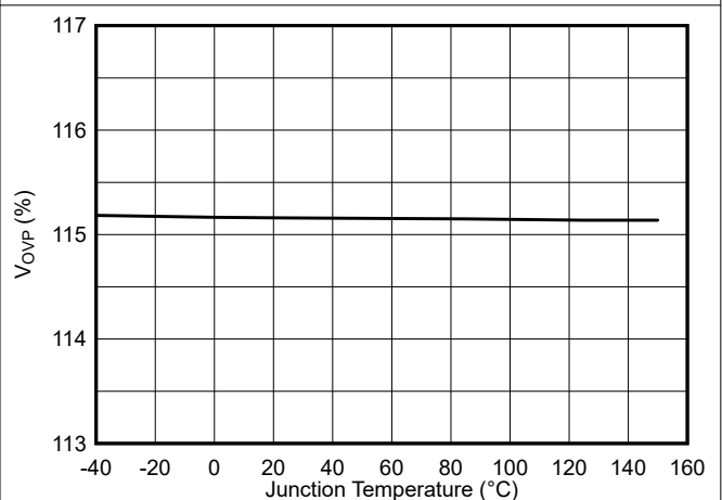
6-12. OVP Threshold vs Junction Temperature
