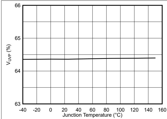
6-13. UVP Threshold vs Junction Temperature
