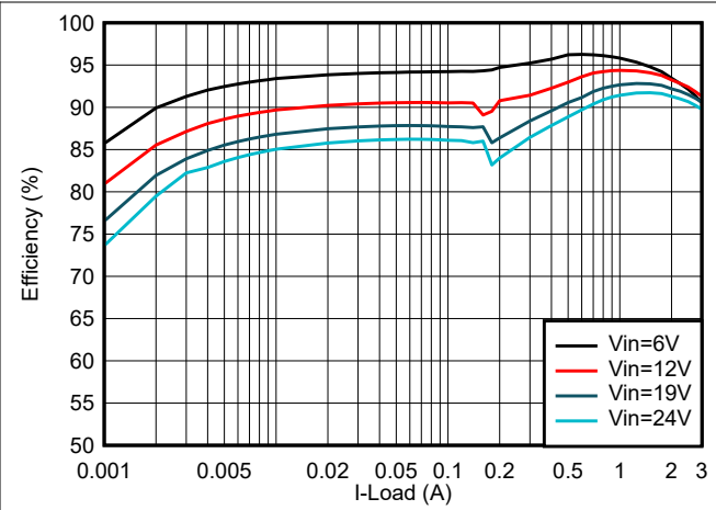
6-14. Efficiency, V_{OUT} = 3.3\text{ V} , f_{SW} = 500\text{ kHz} , L = 4.7\text{ }\mu\text{H}
