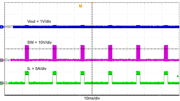
8-21. Output Hard Short Hiccup
