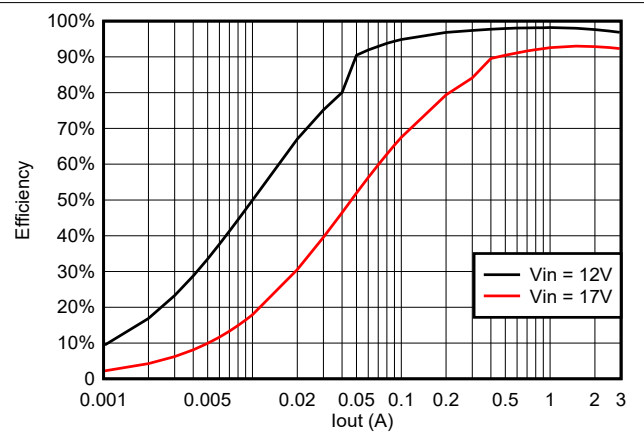
6-20. TPS563257 Efficiency at 10 V OUT with a 4.7-µH Inductor
