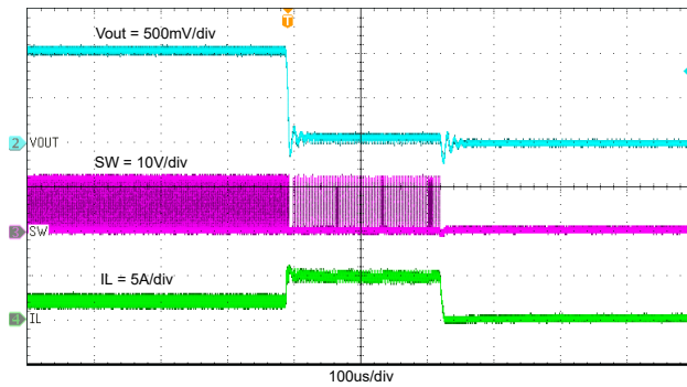
8-20. TPS563257 Normal Operation to Output Hard Short
